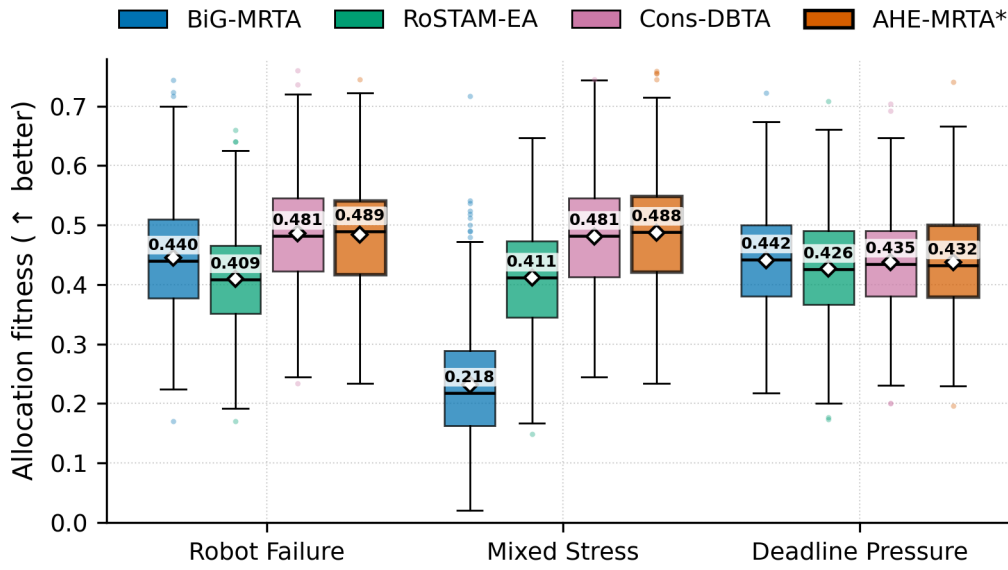
Fig. 4. Navigation-proxy fitness at the primary 5-robot/25-task scale (500 seeds per cell). Boxes show the interquartile range, centre lines the median (value annotated above each box), diamonds the mean, and whiskers 1.5 interquartile ranges; points are outliers. AHE-MRTA and Consensus-DBTA are statistically tied under robot failure and deadline pressure (paired Wilcoxon p \geq 0.391 ); the only significant separation is mixed stress, where AHE-MRTA leads by 0.007 ( p=0.042 ).
