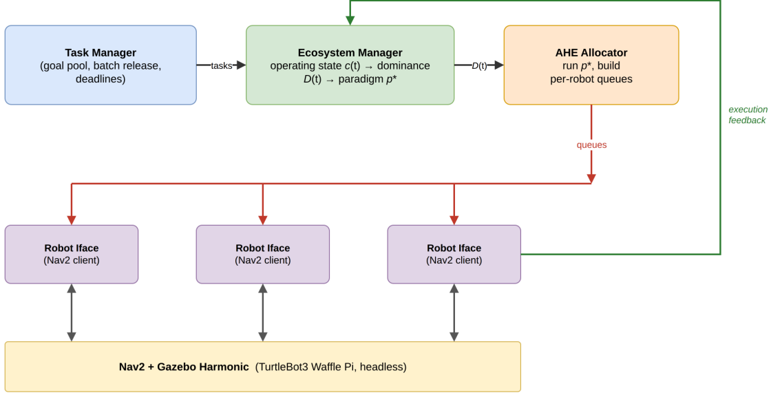
Fig. 2. System architecture. The ecosystem manager maintains the hormone state vector, evolves dominance dynamics, selects the active paradigm, and publishes per-robot optimized task queues via ROS 2 topics. Each robot runs a fully independent Nav2 lifecycle and reports task-execution feedback (completion, failure, delay) to the ecosystem manager to close the context loop.
