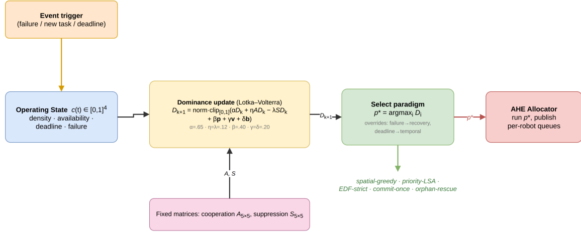
Fig. 1. The Ecosystem-Driven Paradigm Selection mechanism. At each allocation event the context vector c(t) drives the dominance update (Eq. 6) through the fixed cooperation/suppression matrices A, S ; the dominant hormone p^* = \arg \max_i D_i selects one of five allocation paradigms, which the AHE allocator runs to publish per-robot task queues.
