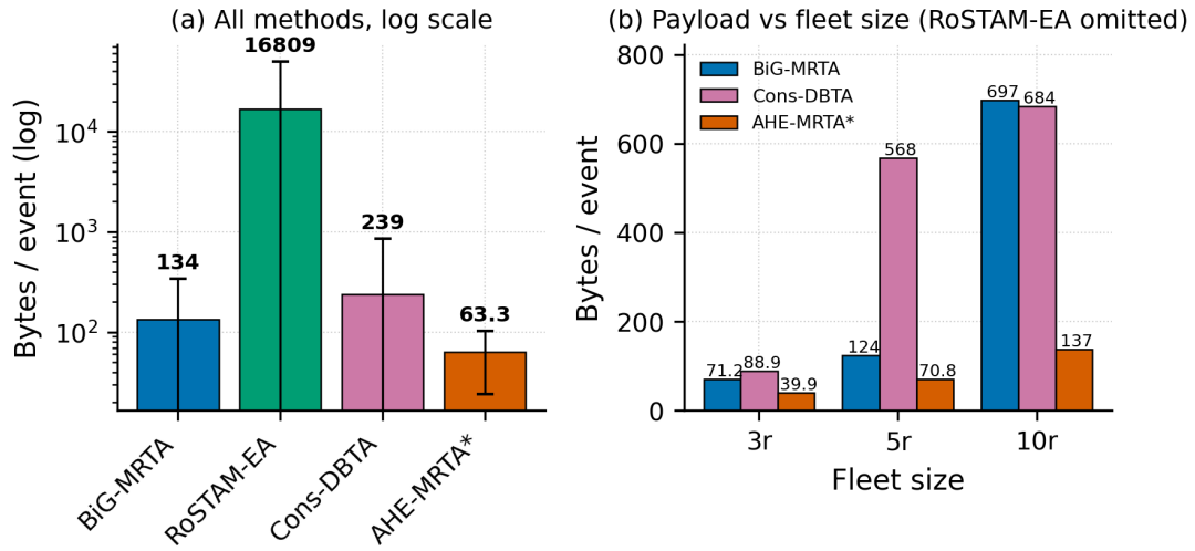
Fig. 13. Communication footprint per allocation event, counted from the fields each protocol transmits. (a) All methods, pooled over scales (log axis). (b) The same payload by fleet size, RoSTAM-EA omitted for range: only per-robot queues are broadcast by AHE-MRTA, so its payload grows linearly in the fleet while bid and utility-matrix exchanges grow with the robot-task product.
