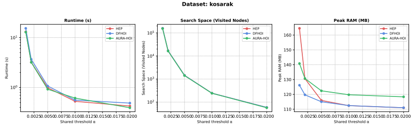
Fig. 3. Runtime and memory scalability across thresholds on large clickstream kosarak .
