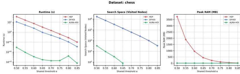
Fig. 2. Runtime and memory scalability across thresholds on chess .
