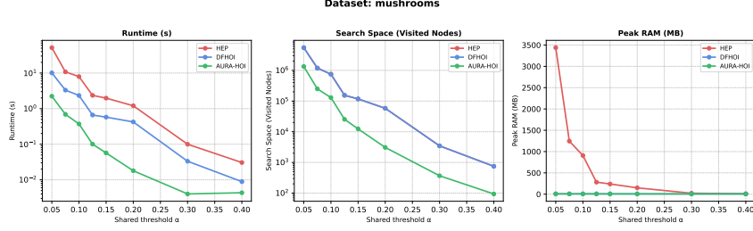
Fig. 1. Runtime and memory scalability across thresholds on mushrooms .
