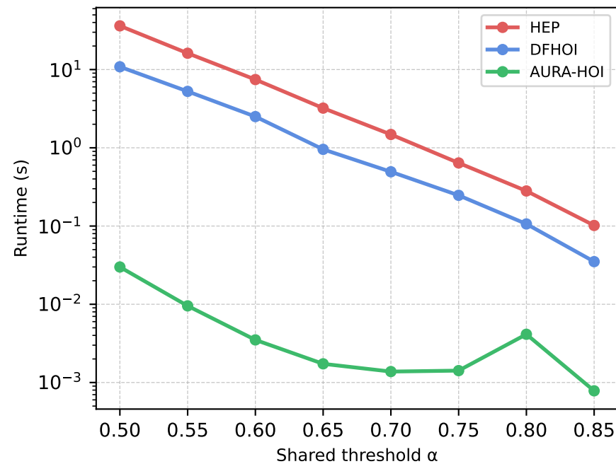
Runtime (s)
