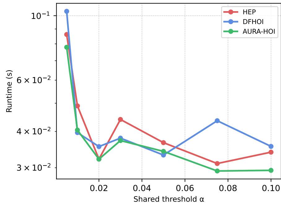
Runtime (s)
