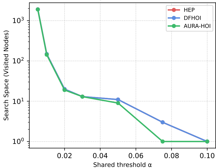
Search Space (Visited Nodes)
