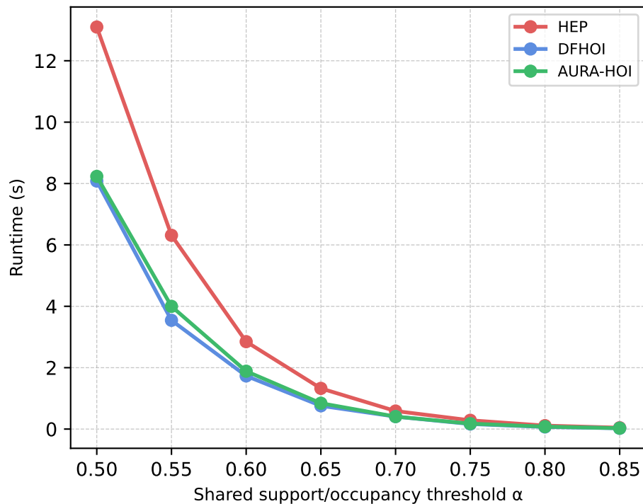
Runtime (s)
