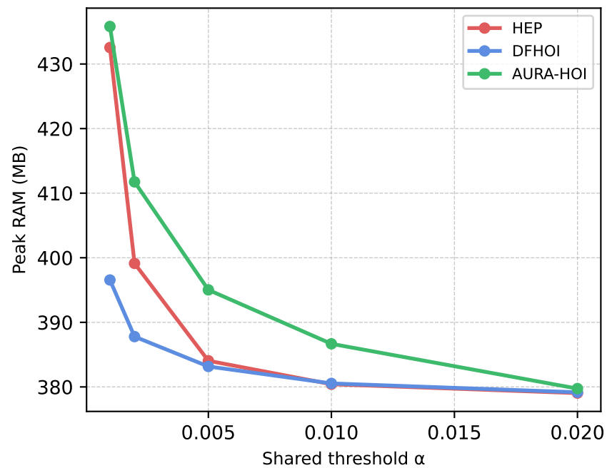
Peak RAM (MB)
