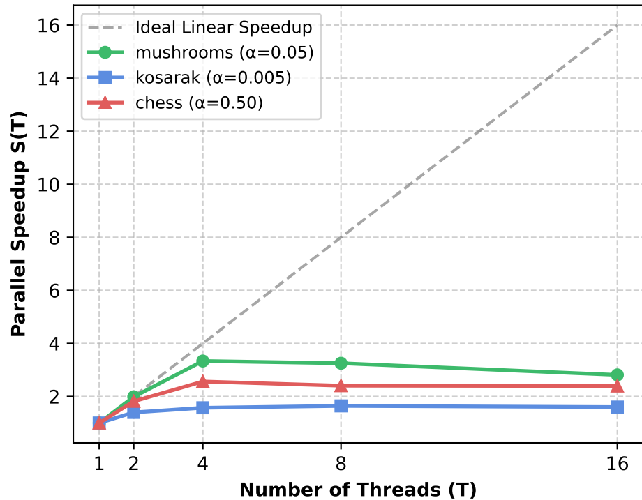
Parallel Scalability Curve
