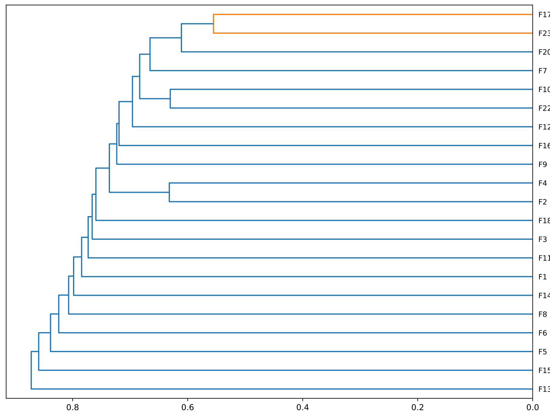
Kinship-Based Clustering (Dendrogram)
