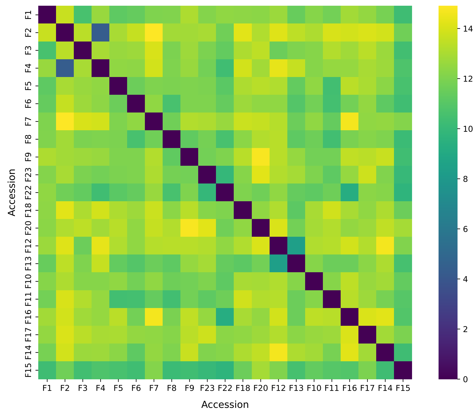
Genetic Distance Matrix (150 SNPs)
