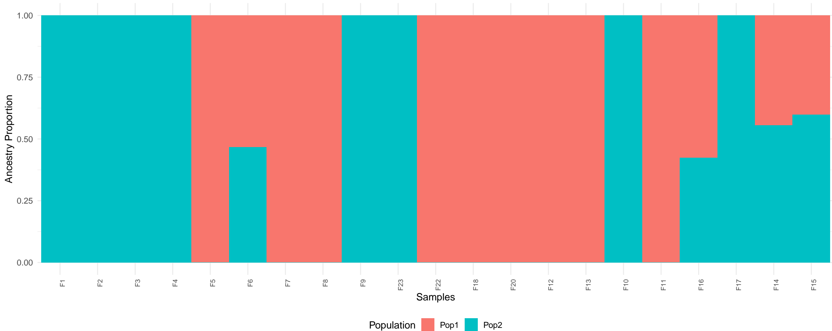
Admixture Proportions – K = 2 (BEST)
