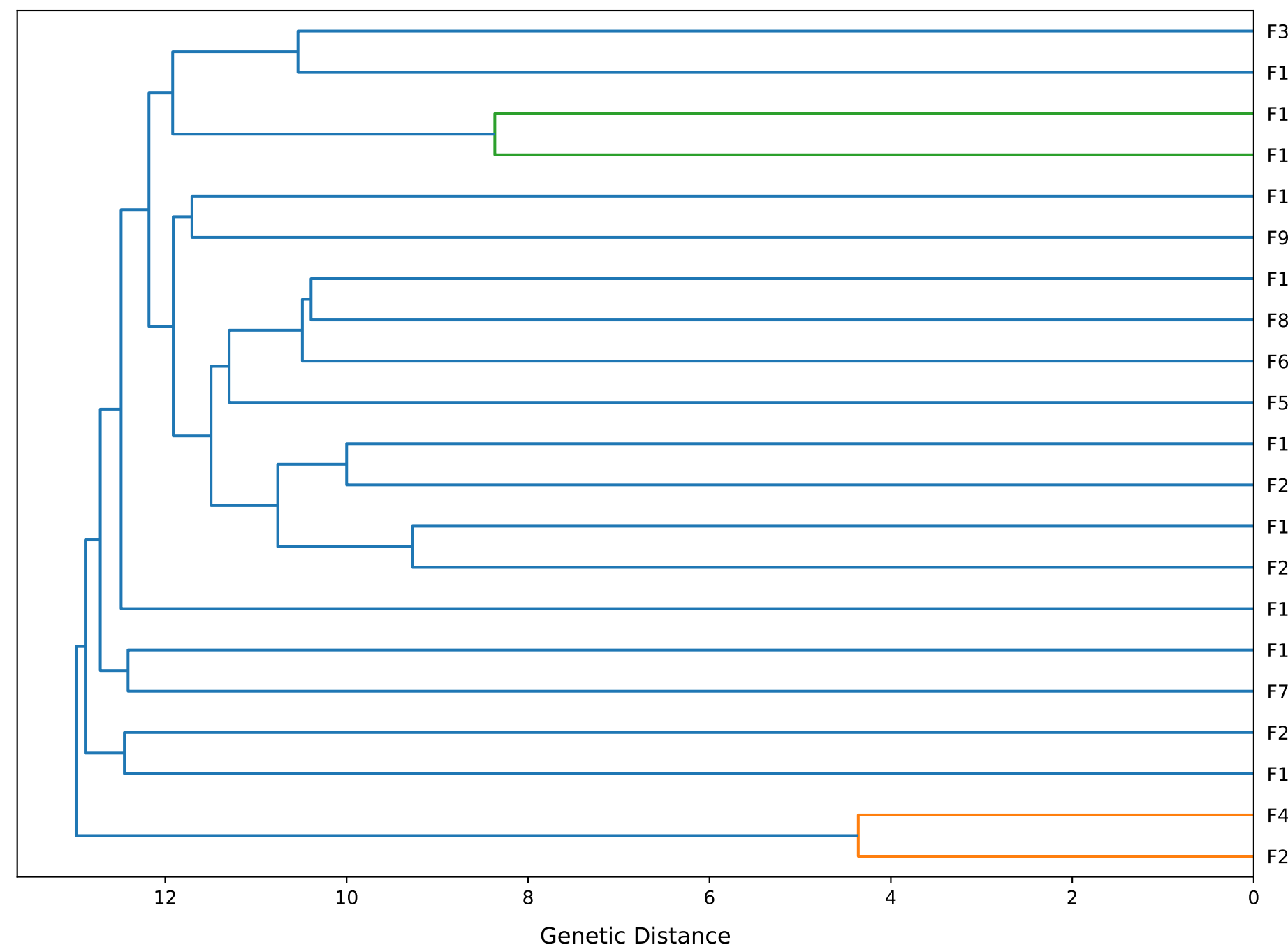
Phylogenetic Tree (Ward Linkage)
