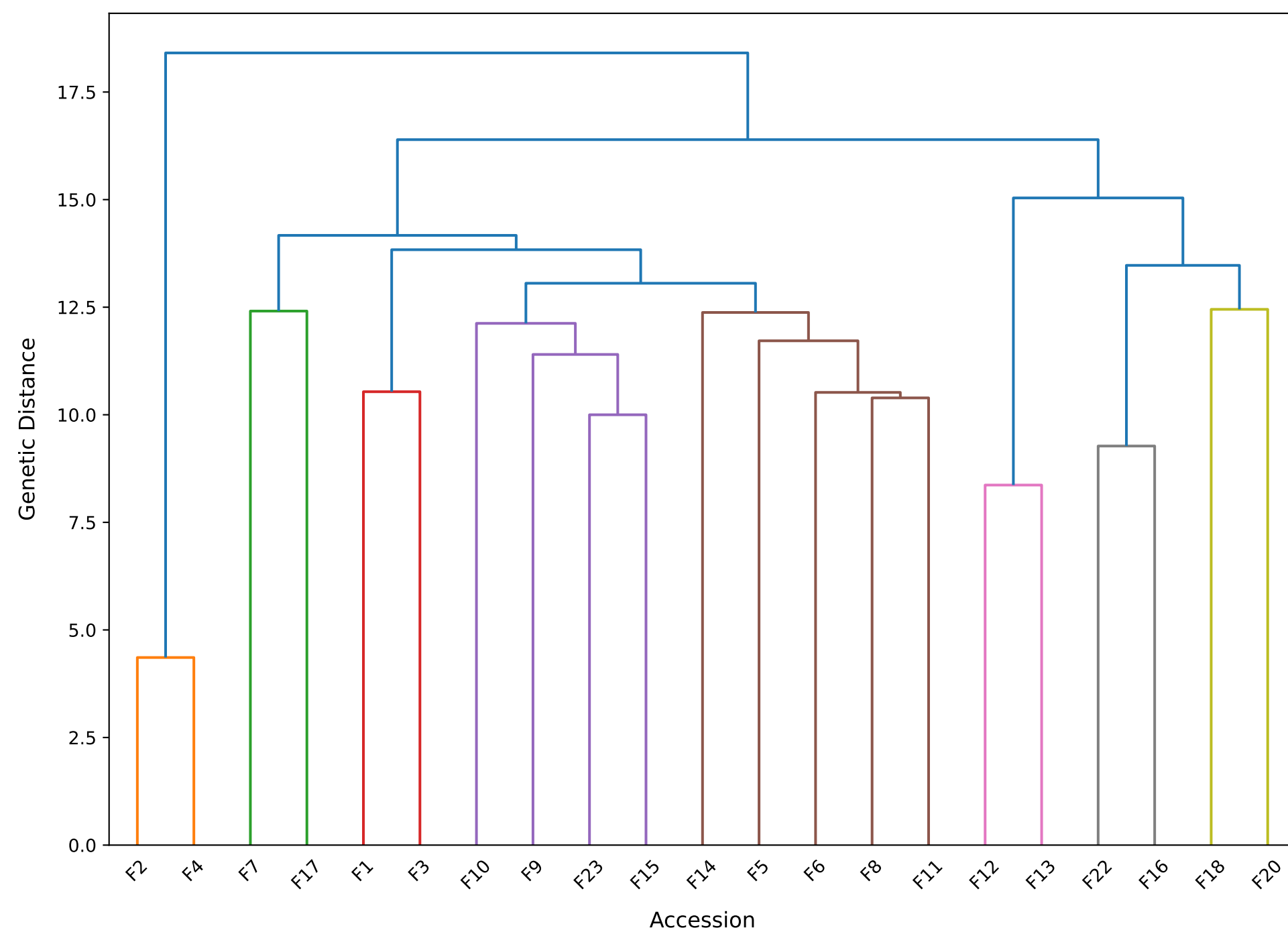
Phylogenetic Tree (Ward Linkage)
