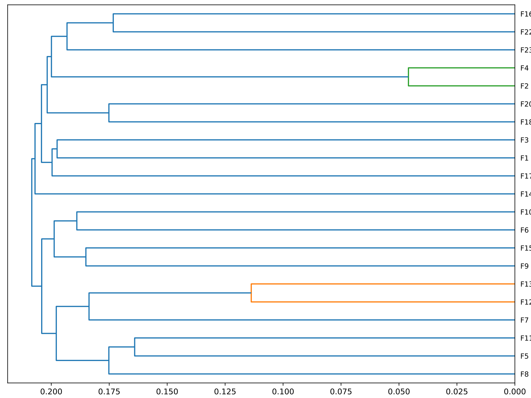
IBS-Based Clustering (Dendrogram)
