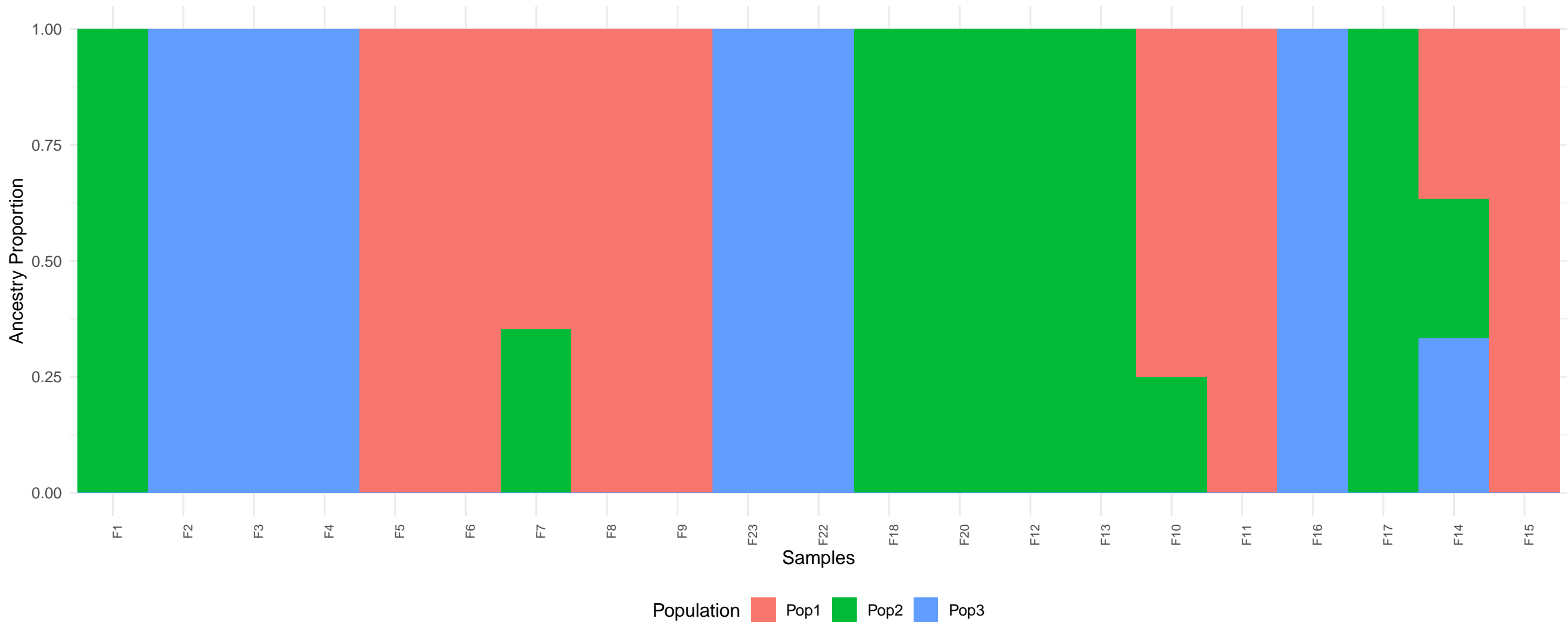
Admixture Proportions – K = 3
