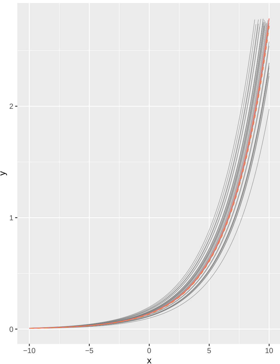
Random intercept
