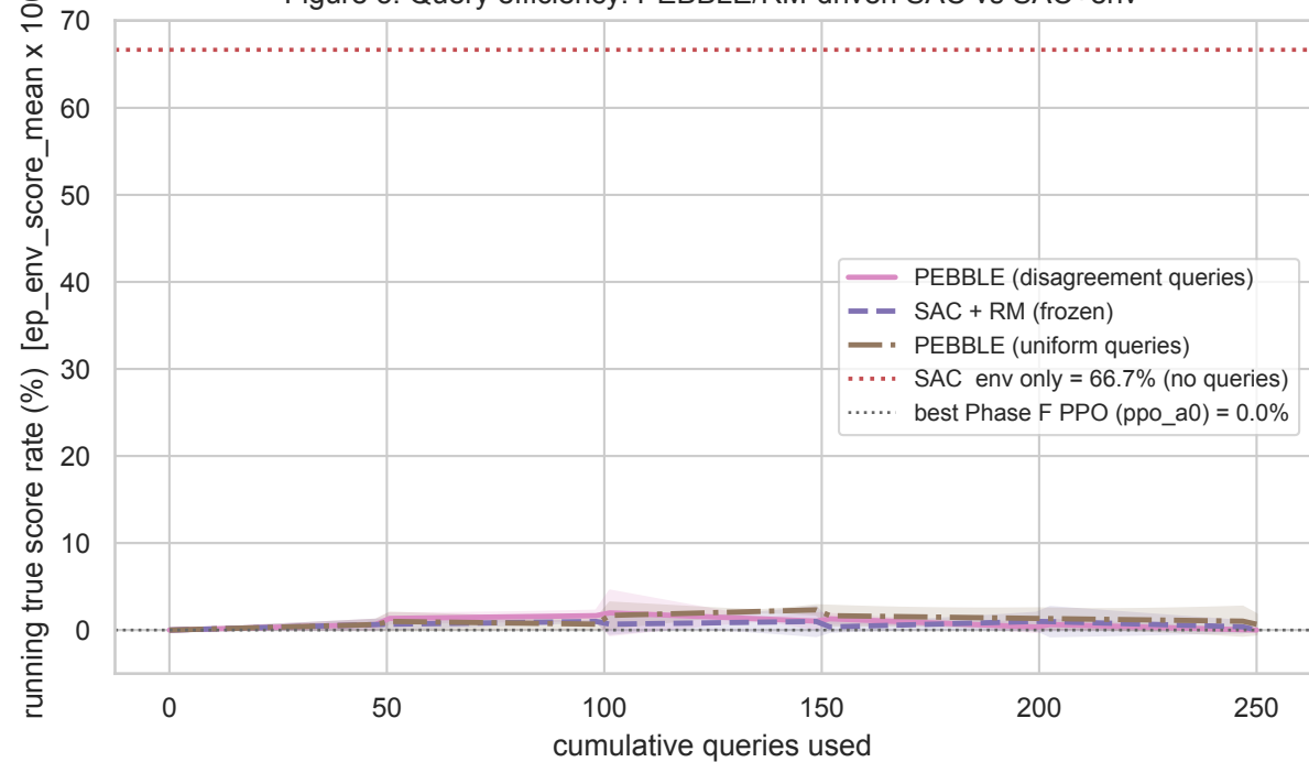
Figure 5. Query efficiency: PEBBLE/RM-driven SAC vs SAC+env
