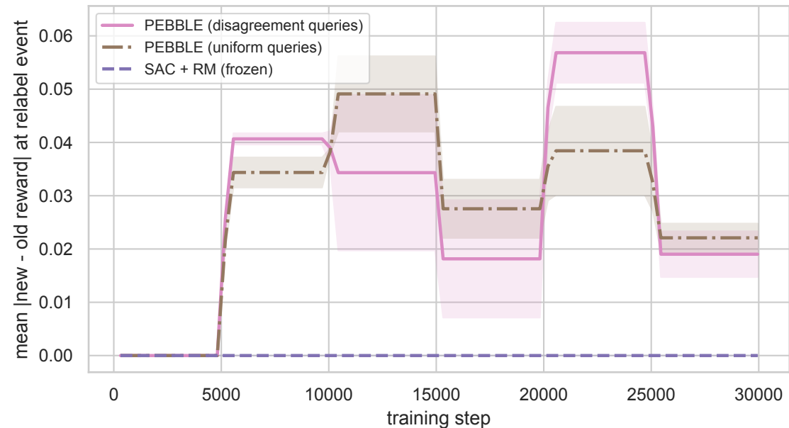
Figure 6. Replay relabeling moves the reward signal
