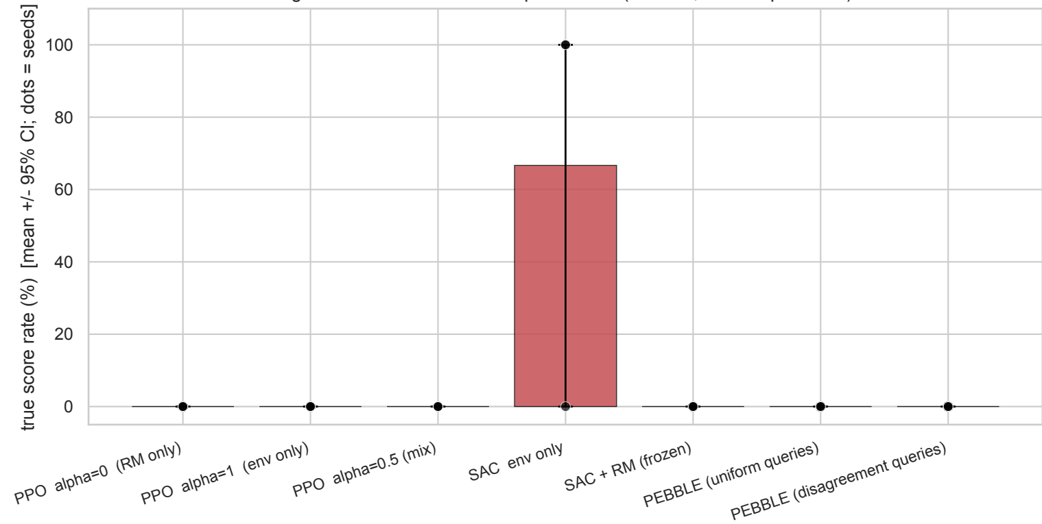
Figure 7. Final true-score rate per method (3 seeds, bootstrap 95% CI)
