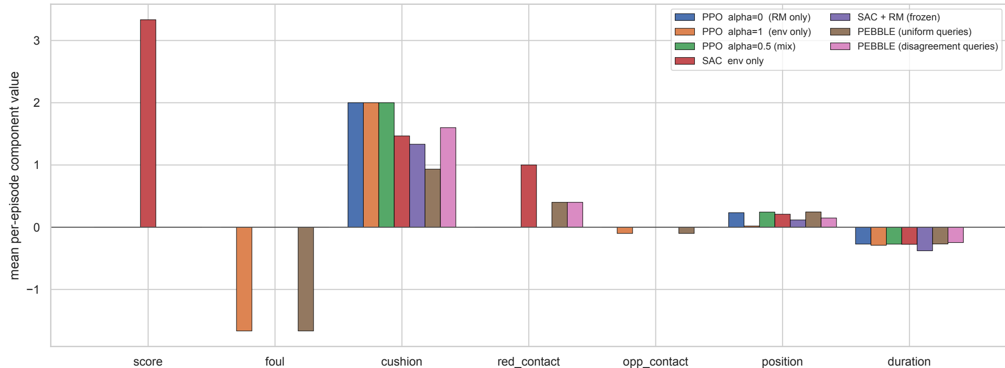
Figure 8. Component attribution: only sac_env activates `score`; PEBBLE stuck in cushion subspace
