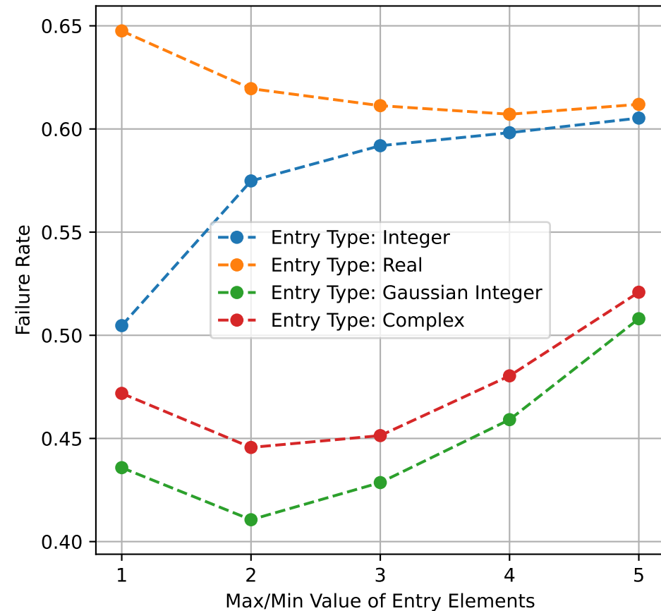
Tolerance = 1e-15
