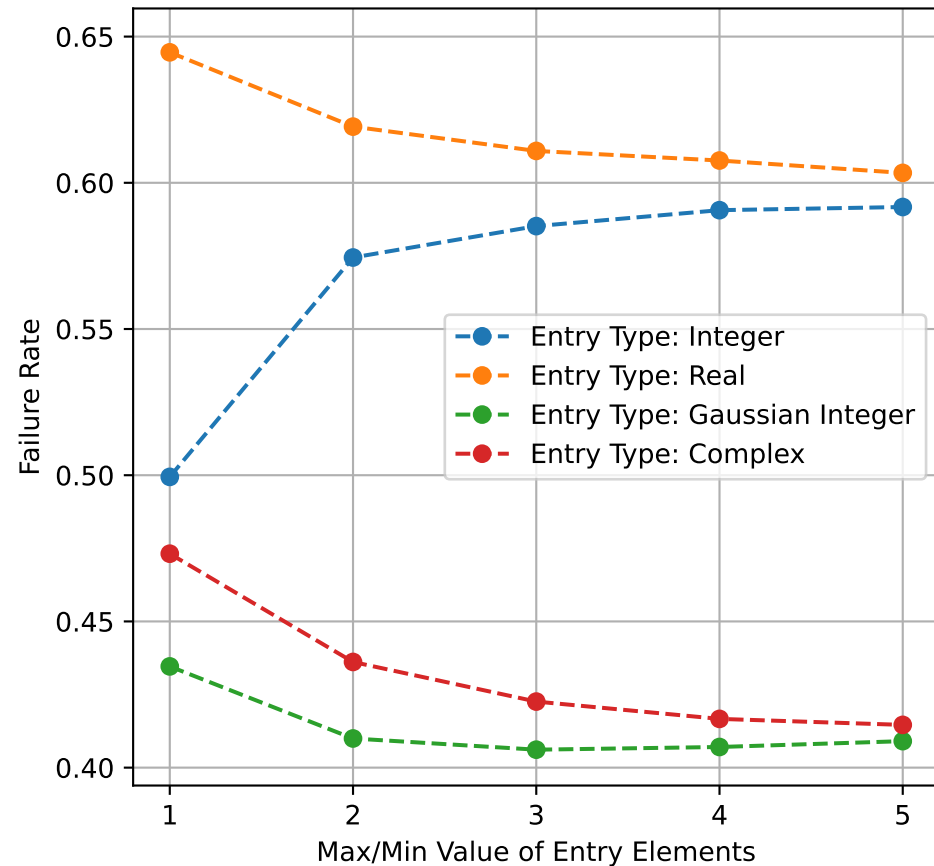
Tolerance = 1e-5
