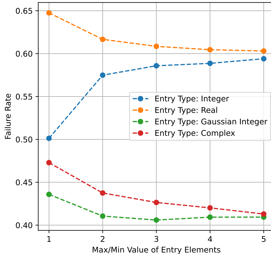
Tolerance = 1e-10
