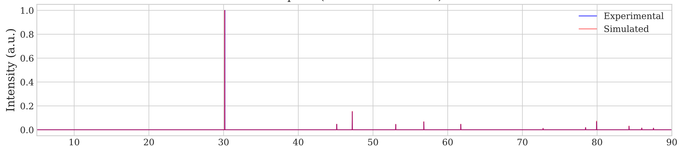
Tamarugite (DTW Distance: 4.51)
