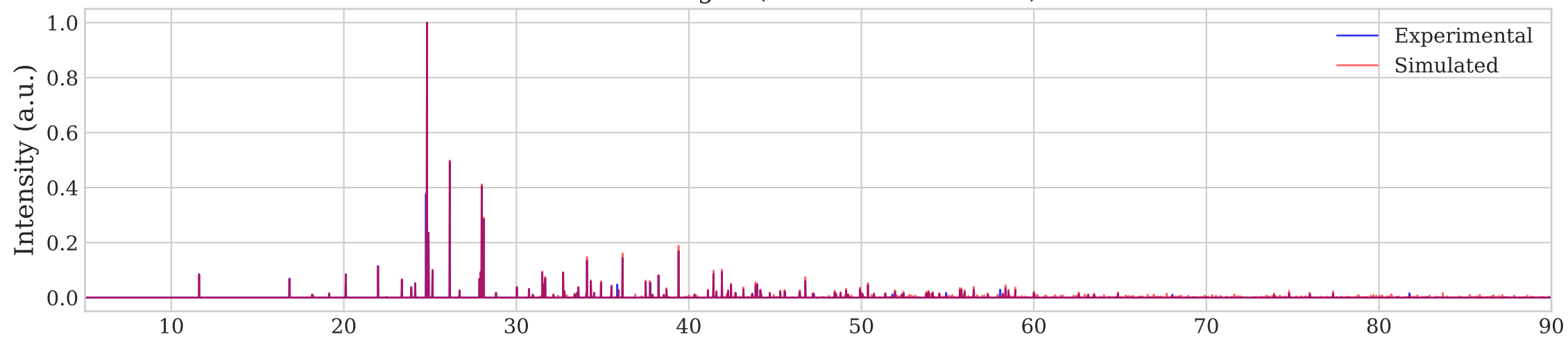
Chalcophyllite (DTW Distance: 9.00)
