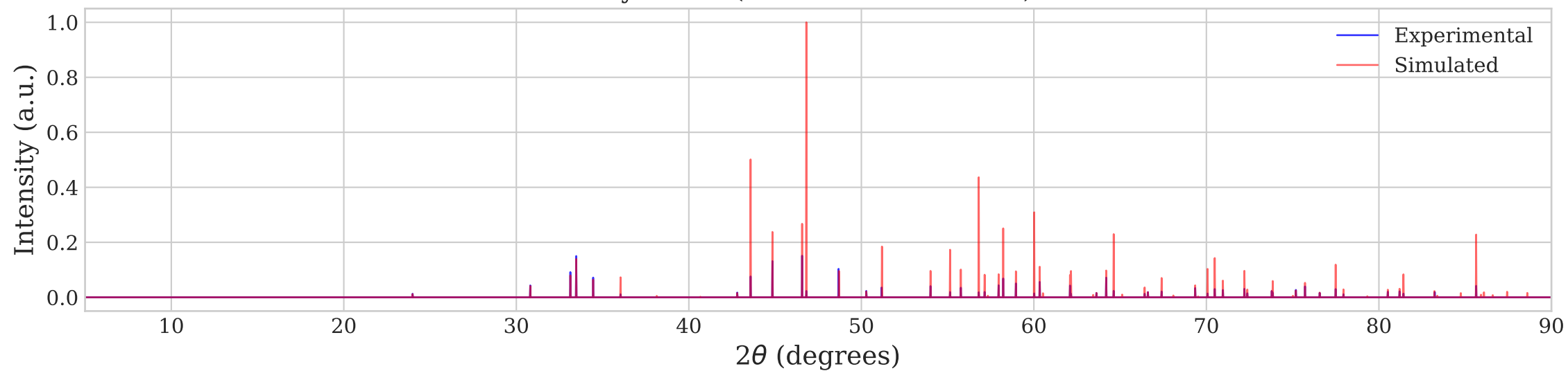
Pyroxene (DTW Distance: 47.35)
