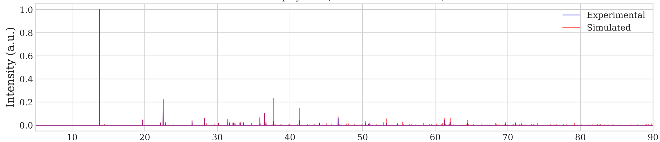
Pyroxene (DTW Distance: 47.35)
