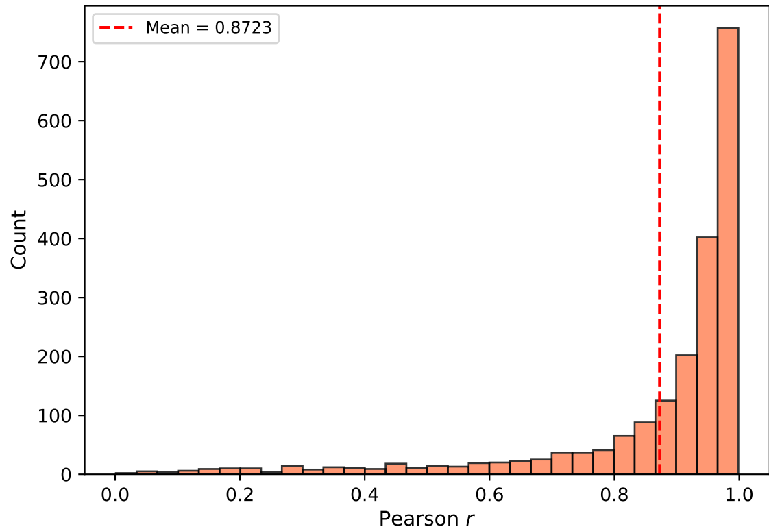
Pearson correlation distribution
