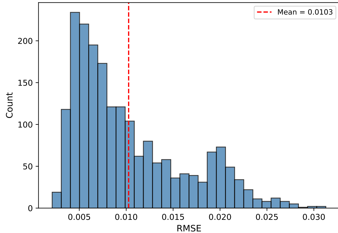
RMSE distribution (model output vs measured)
