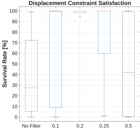
Fig. 7. Survival rate representing the compliance with the \pm 2.5m physical displacement constraint.
