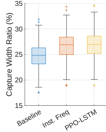
Fig. 8. Comparison of Capture Width Ratio (CWR) distributions across 200 validation irregular wave scenarios.
