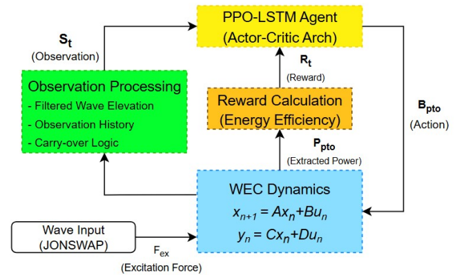
Fig. 1. Block diagram of the proposed PPO-LSTM control system for the Wave Energy Converter
