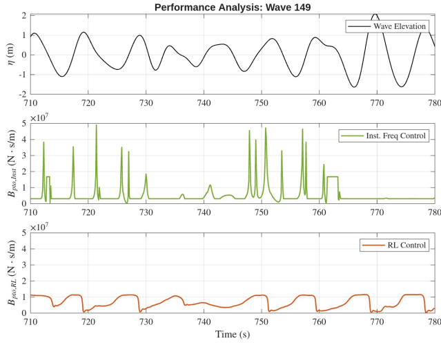
Fig. 9. Time-series control behavior under irregular wave scenario 149: (a) wave elevation, (b) damping coefficient command of the IF controller, and (c) damping coefficient command of the proposed PPO-LSTM controller.
