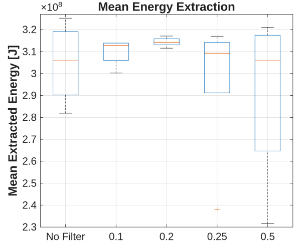
Fig. 6. Distribution of mean extracted energy across 200 validation wave scenarios for the 'No filter' baseline and different filter bandwidth ratios ( r ).
