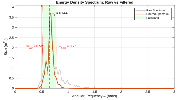
Fig. 5. Energy density spectrum of Sea State 5 comparing raw and filtered signals ( r = 0.2 ).
