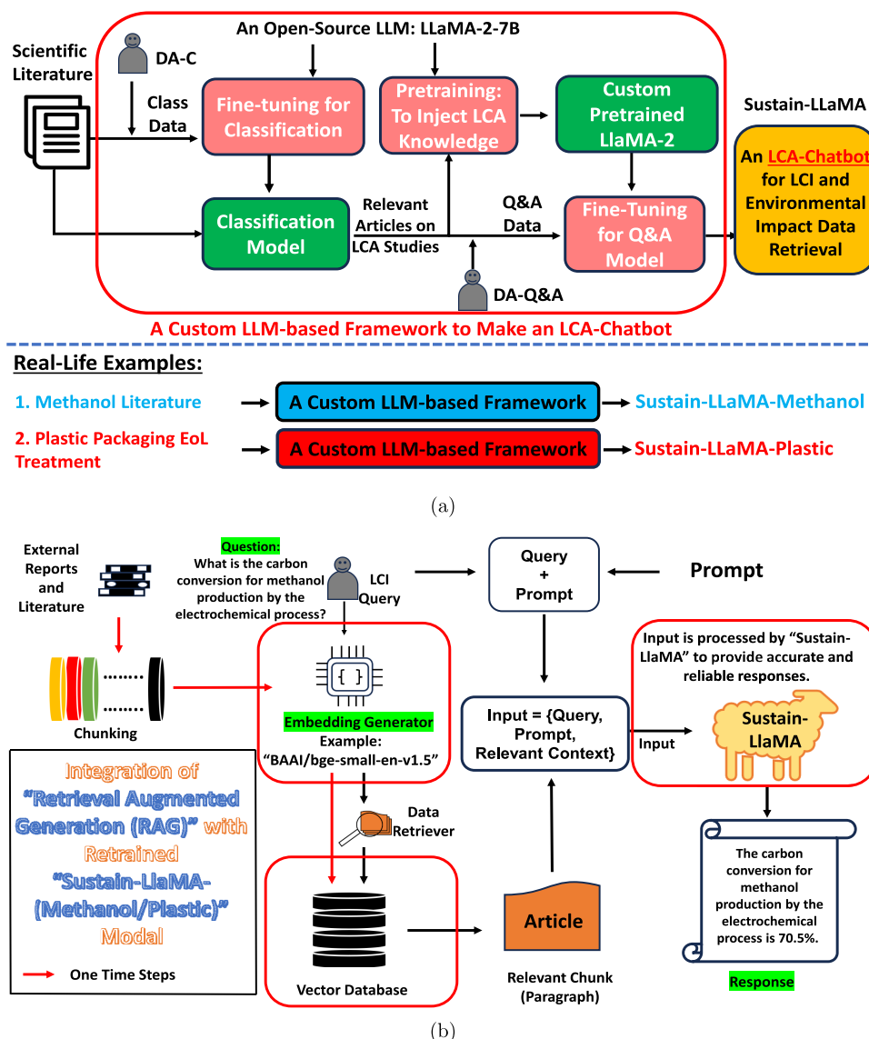
Figure 1. These two figures illustrate (a) a structured retraining workflow to develop Sustain-LLaMA, fine-tuning for classification, pretraining for domain knowledge injection, and fine-tuning for Q&A applied to LLaMA-2-7B using annotated LCA and environmental data sets from two case studies: methanol and plastic packaging end-of-life treatment. (b) A schematic of the RAG system with an LLM: uploaded documents (PDF/TXT) are chunked, vectorized via an embedding generator, and stored in a vector database. An input query is embedded, and relevant chunks are retrieved by a data retriever. The query and retrieved content are then processed by Sustain-LLaMA to generate a source-grounded response.
