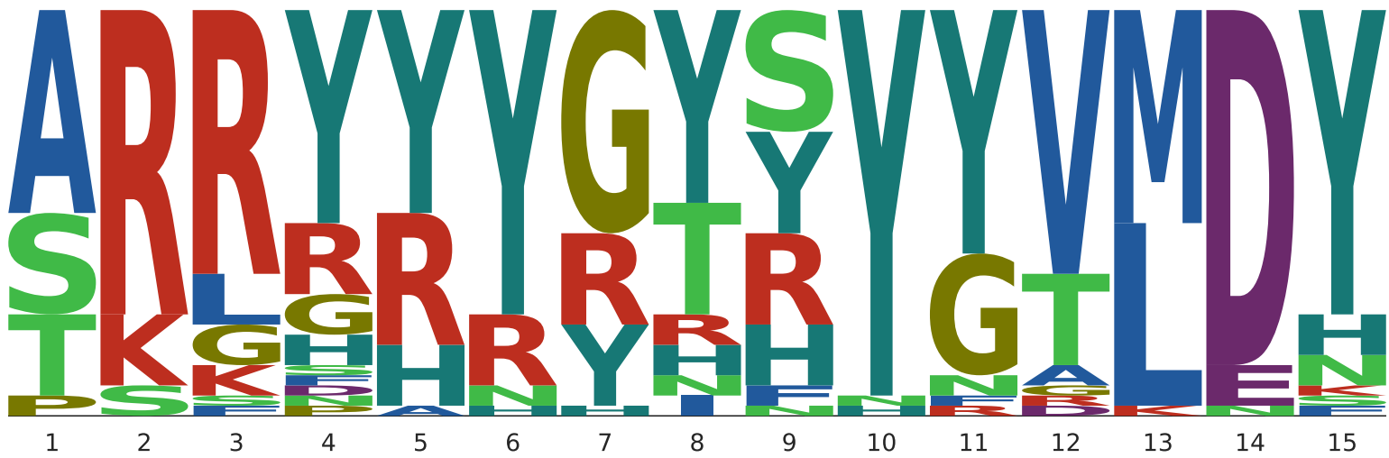
1OB1
