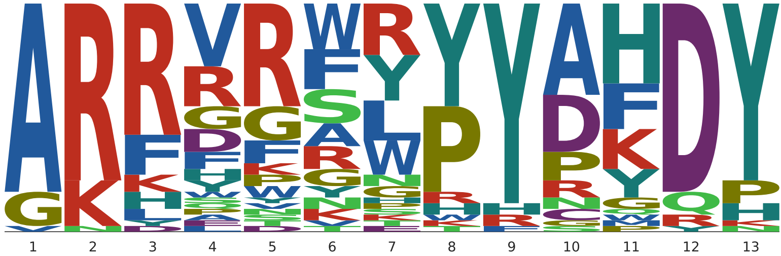
1FBI
