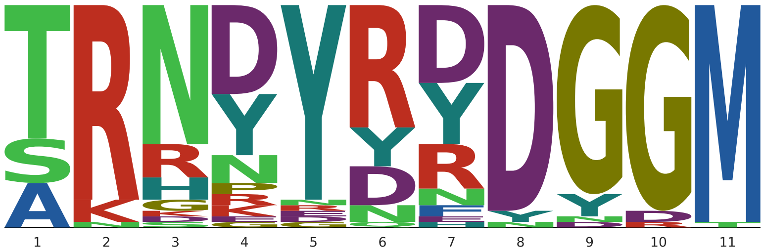
3RAJ
