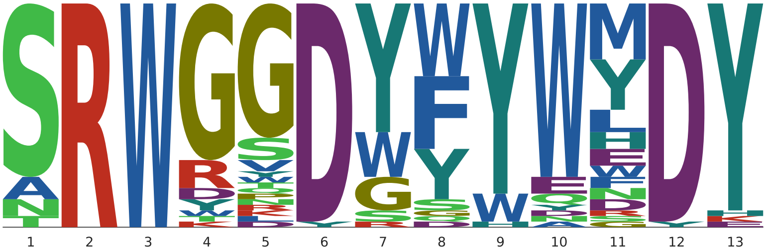
1ADQ
