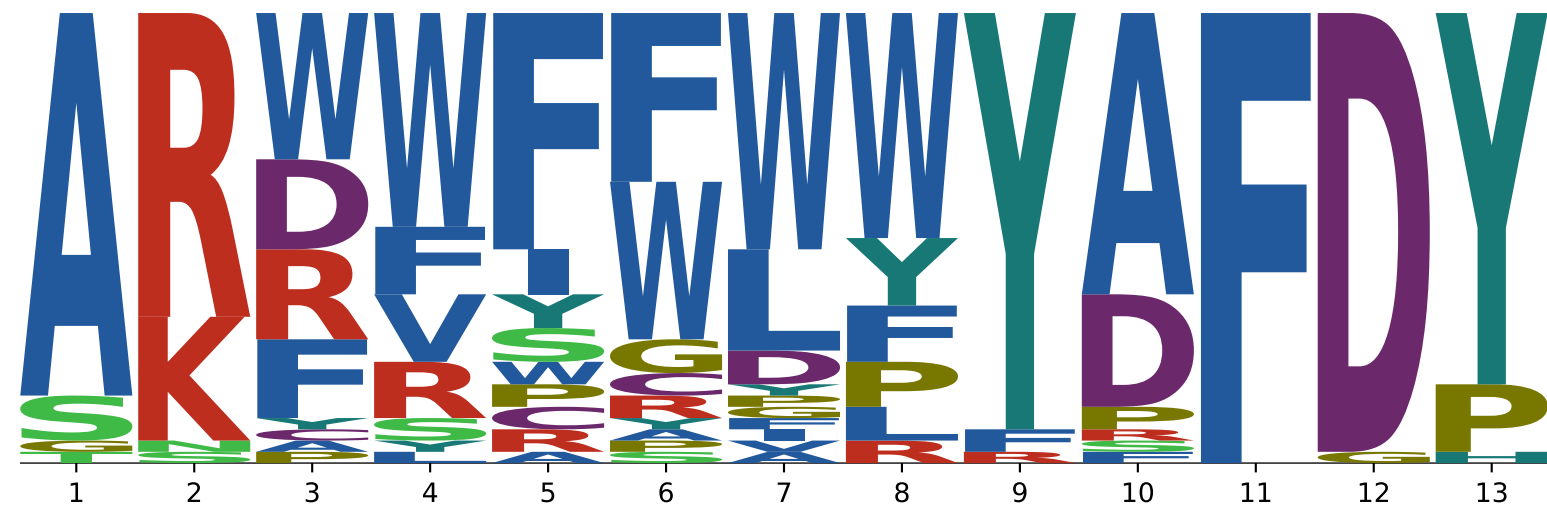
1FBI
