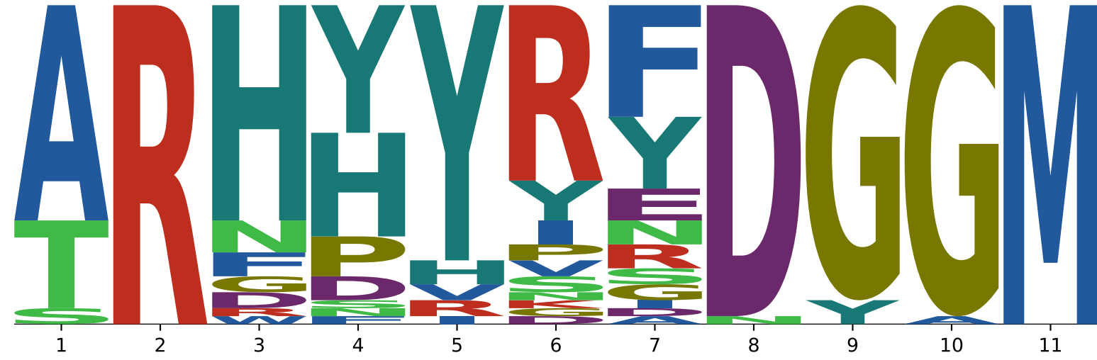
3RAJ
