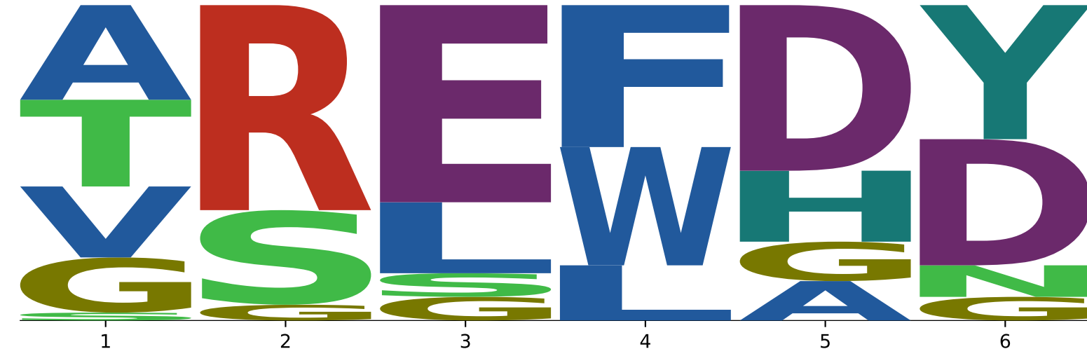
2YPV
