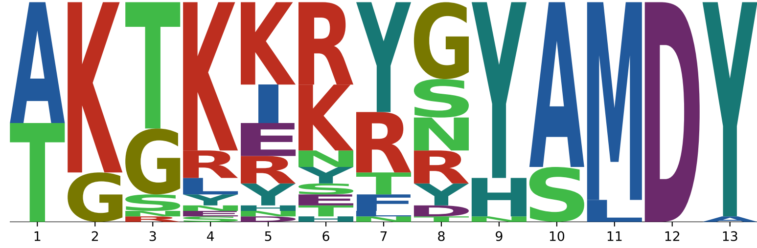
1S78
