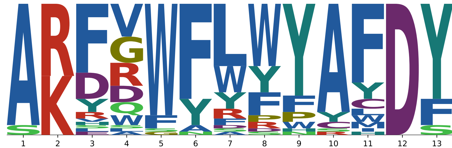
1H0D
