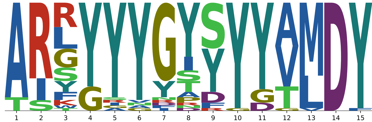
1OB1
