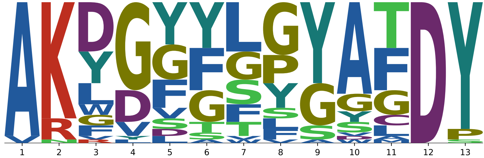
1H0D
