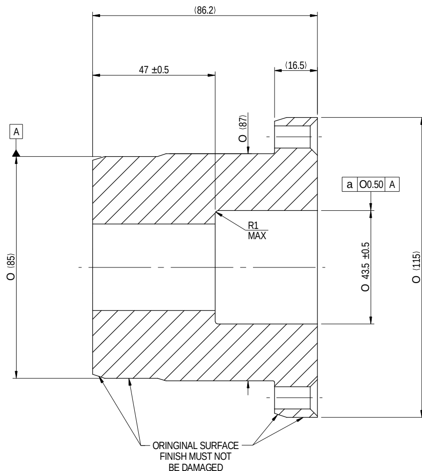
SECTION Z-Z
