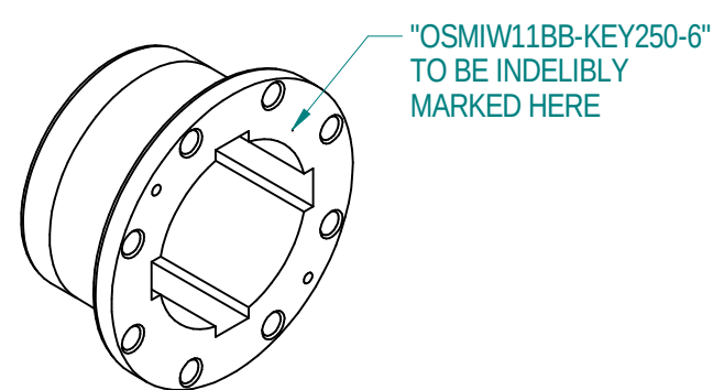
ISOMETRIC VIEW 1:10
