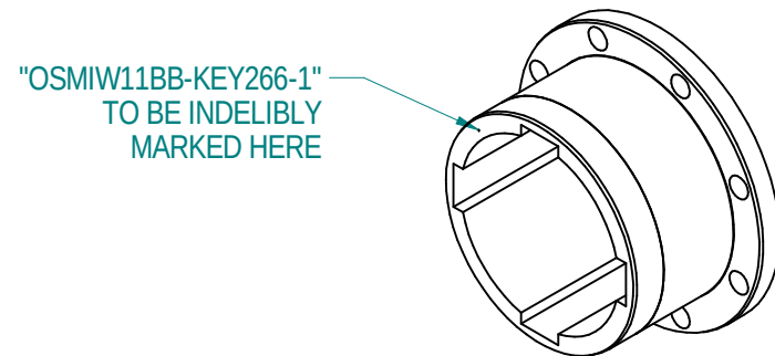
ISOMETRIC VIEW 1:10
