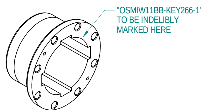
ISOMETRIC VIEW 1:10
