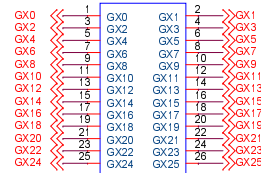
J21 2X13, 2.54 HEADER
