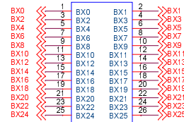
J22 2X13, 2.54 HEADER
