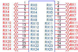
J20 2X13, 2.54 HEADER
