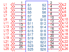
J18 2X13, 2.54 HEADER
