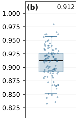
Average precision
