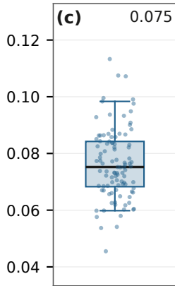
Brier score
