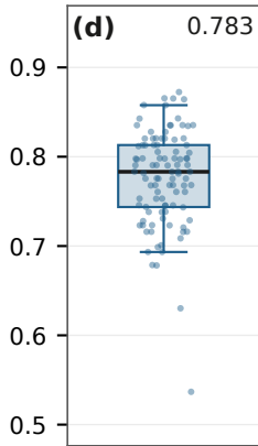
Hanssen-Kuipers score
