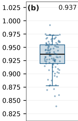
Average precision
