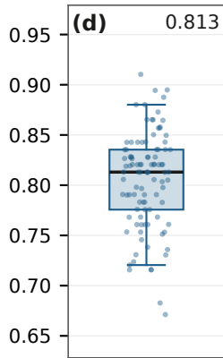
Hanssen-Kuipers score
