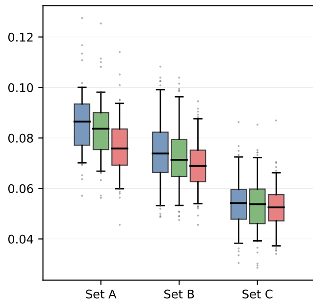
Brier score
