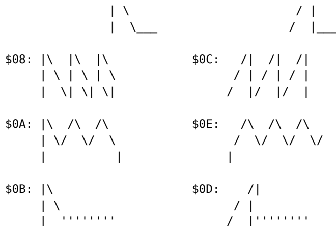
AY-3-8910 Envelope Shapes (R13)
