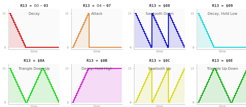
Figure 26: AY envelope shape waveforms
