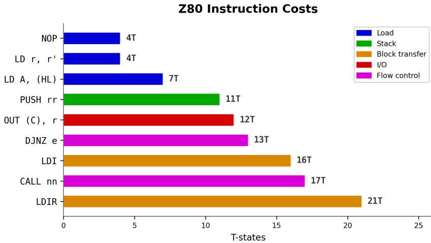
Figure 1: T-state costs for common Z80 instructions
