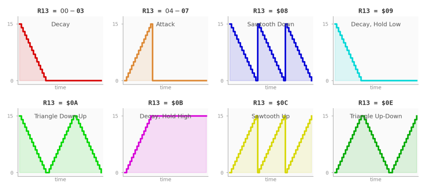
Figure 26: AY envelope shape waveforms
