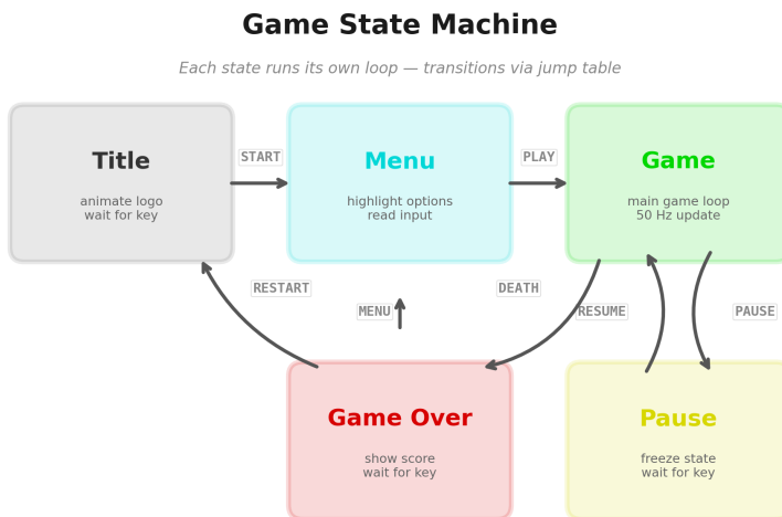
Figure 43: Game state machine: Title, Menu, Game, Pause, and Game Over states connected by labelled transitions. Each state runs its own loop; transitions happen via a jump table.
