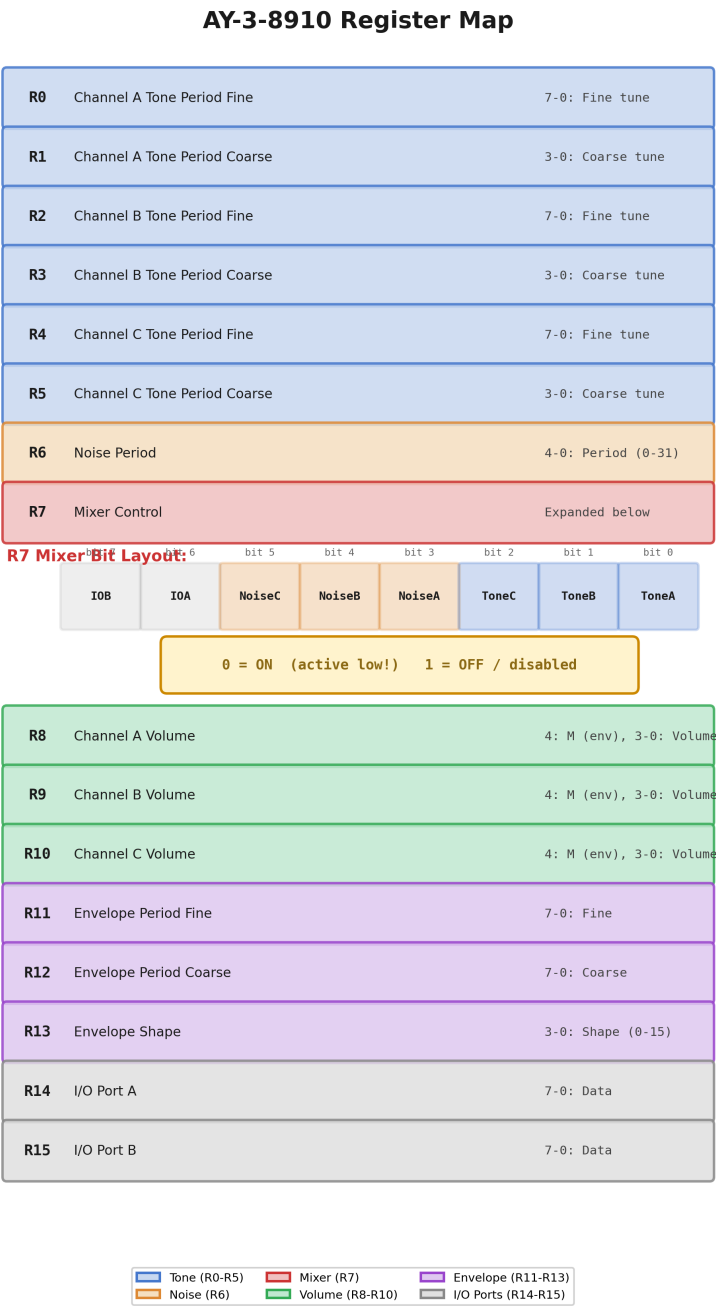
Figure 25: AY-3-8910 register map
