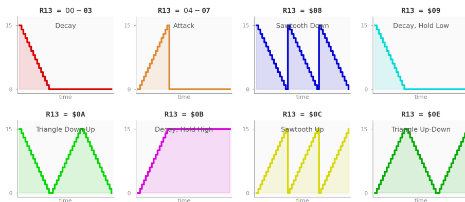
AY envelope shape waveforms
