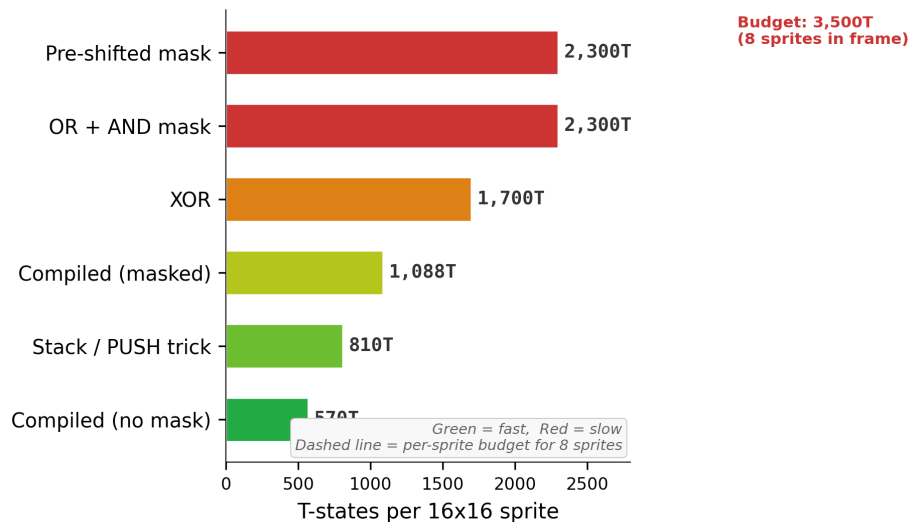
Sprite rendering methods comparison
