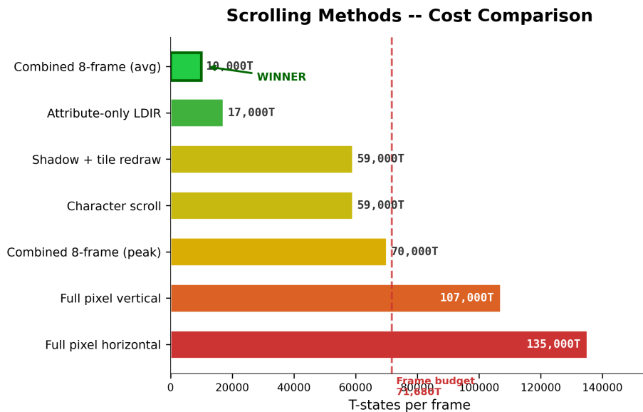
Scrolling technique cost comparison
