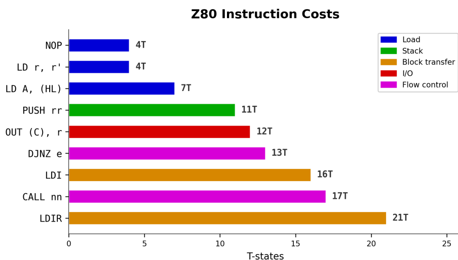
T-state costs for common Z80 instructions
