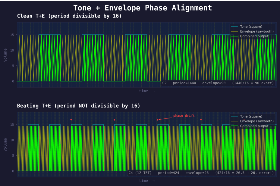
Tone + Envelope Phase Alignment: clean T+E with period divisible by 16 (top) vs beating T+E with rounding error (bottom)
