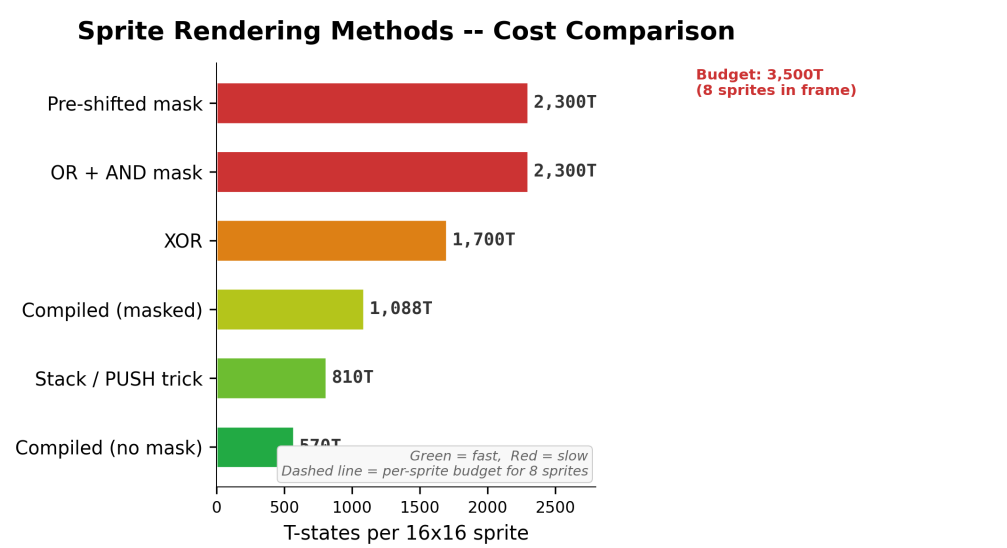
Figure 37: Sprite rendering methods comparison
