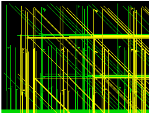
Windblown Trees
