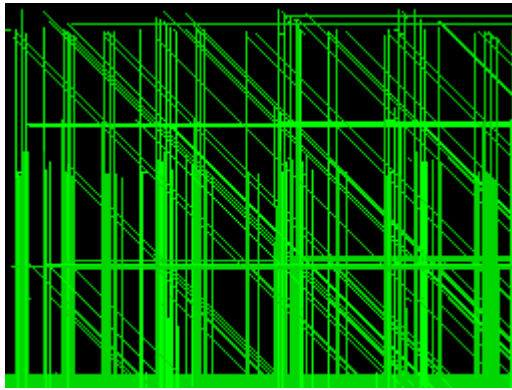
L-System Forest
