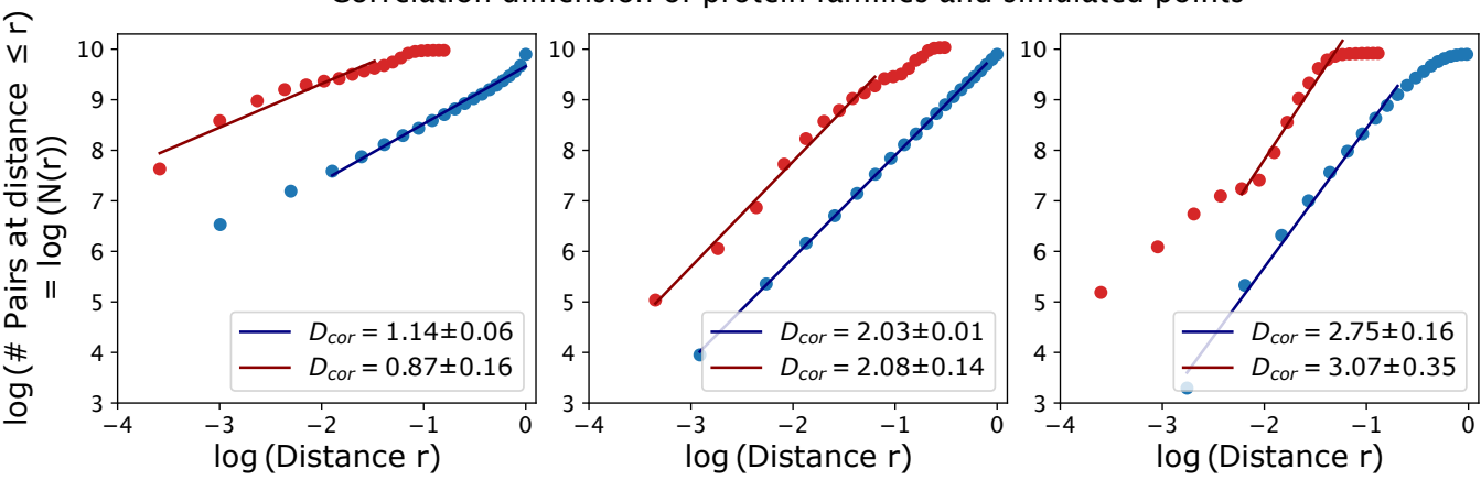
Correlation dimension of protein families and simulated points
