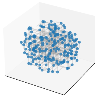
'3D' family: EntOG2107
