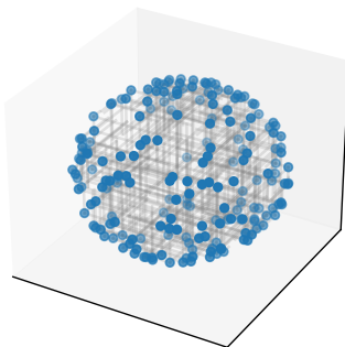
'2D' family: EntOG1310
