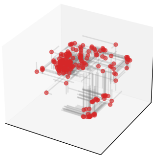
Correlation dimension of protein families and simulated points
