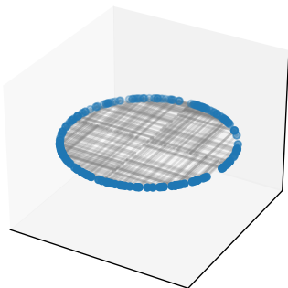
'1D' family: EntOG1922
