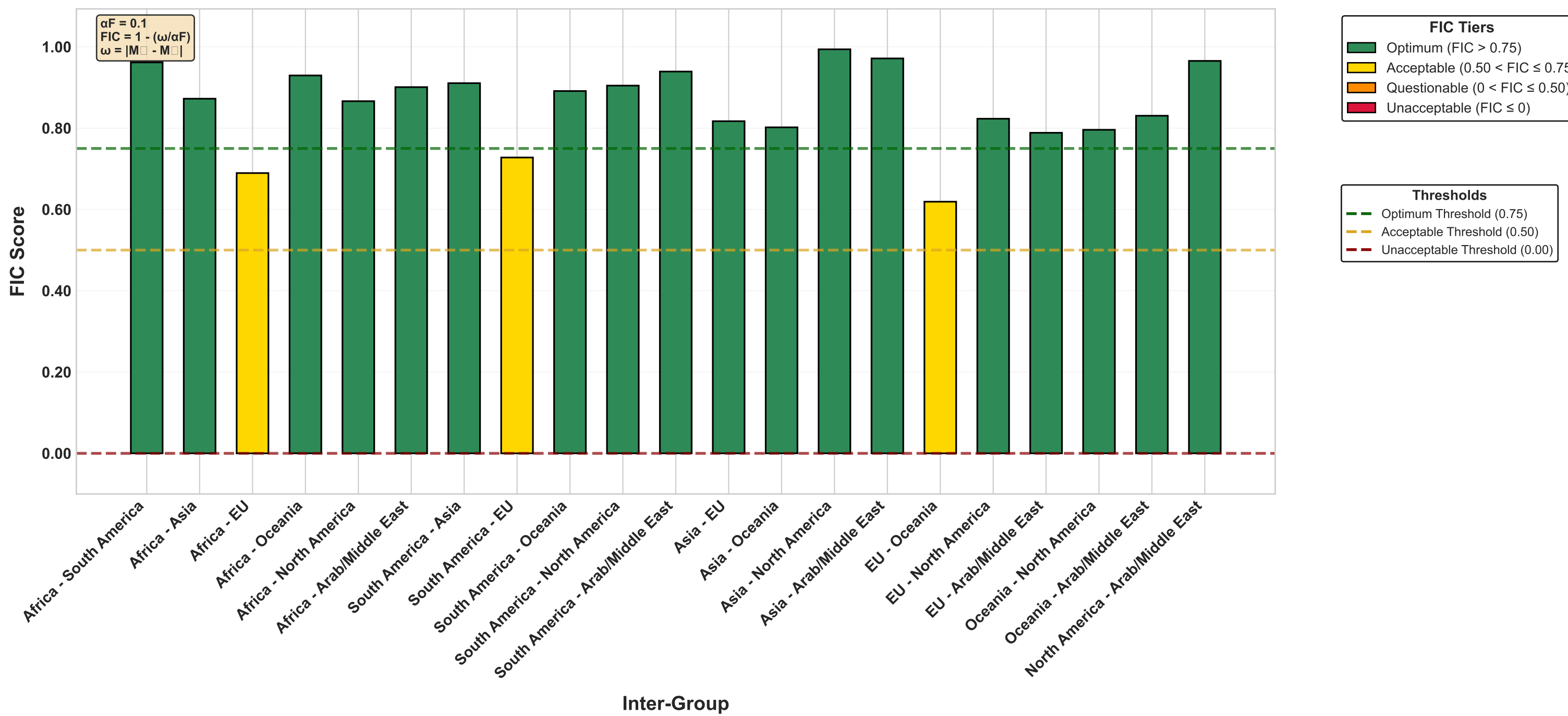
Case2_Criminal Justice - Recidivism Risk_fnr FIC Benchmarking Tiers (fnr, αF = 0.1)
