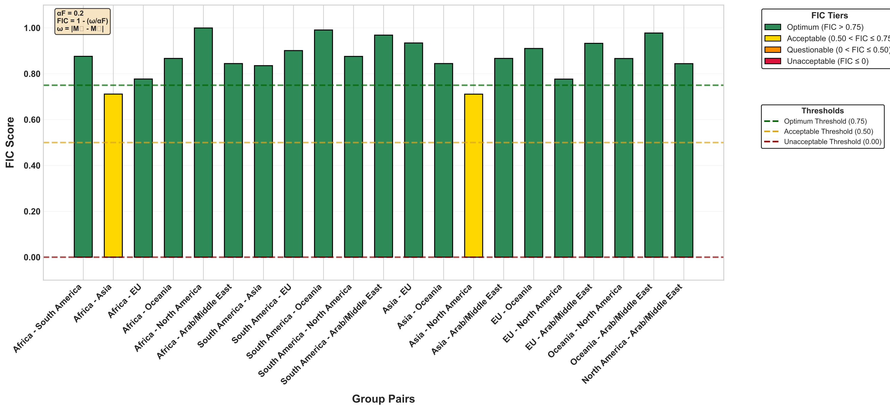
Case2_Criminal Justice - Recidivism Risk_auc FIC Benchmarking Tiers (auc, αF = 0.2)
