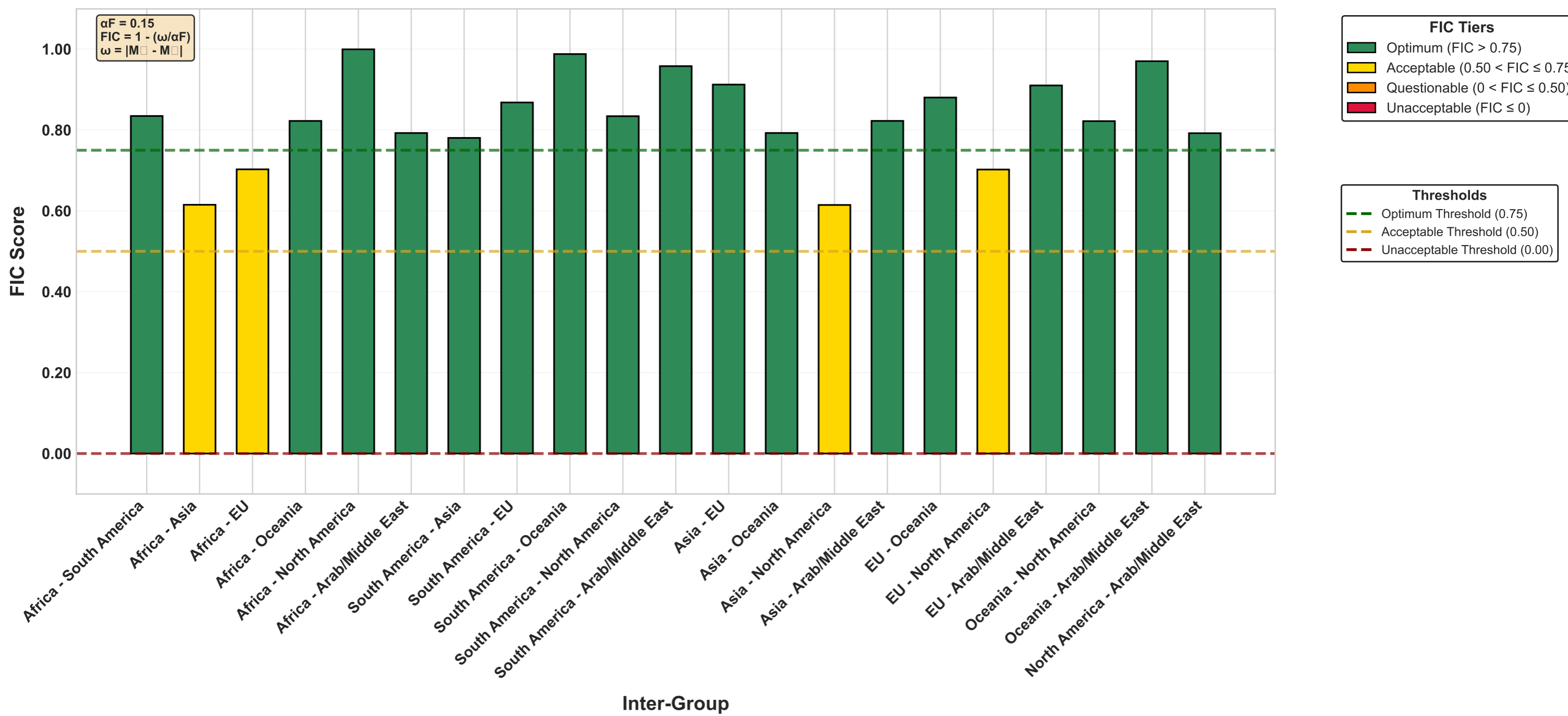
Case2_Criminal Justice - Recidivism Risk_auc FIC Benchmarking Tiers (auc, αF = 0.15)
