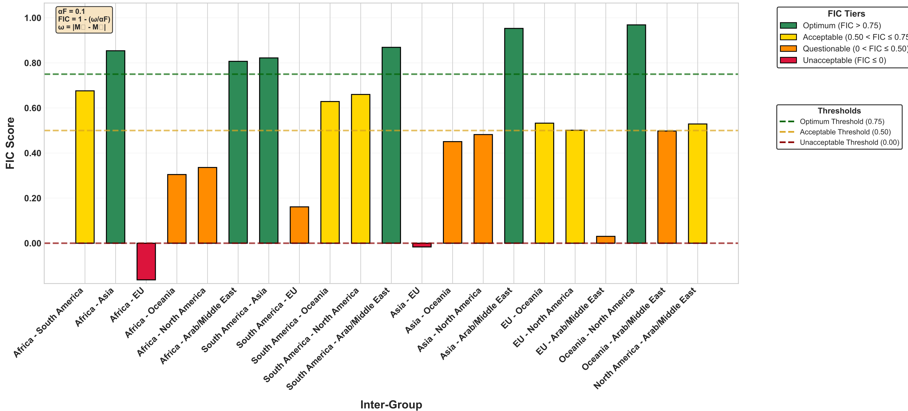
Case2_Criminal Justice - Recidivism Risk_npv FIC Benchmarking Tiers (npv, \alpha F = 0.1 )
