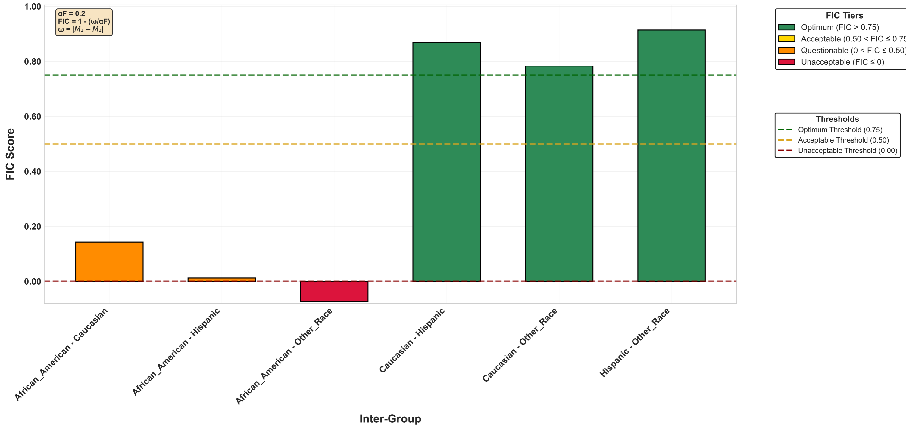
FIC Benchmarking Tiers (selection_rate, \alpha F = 0.2 )
