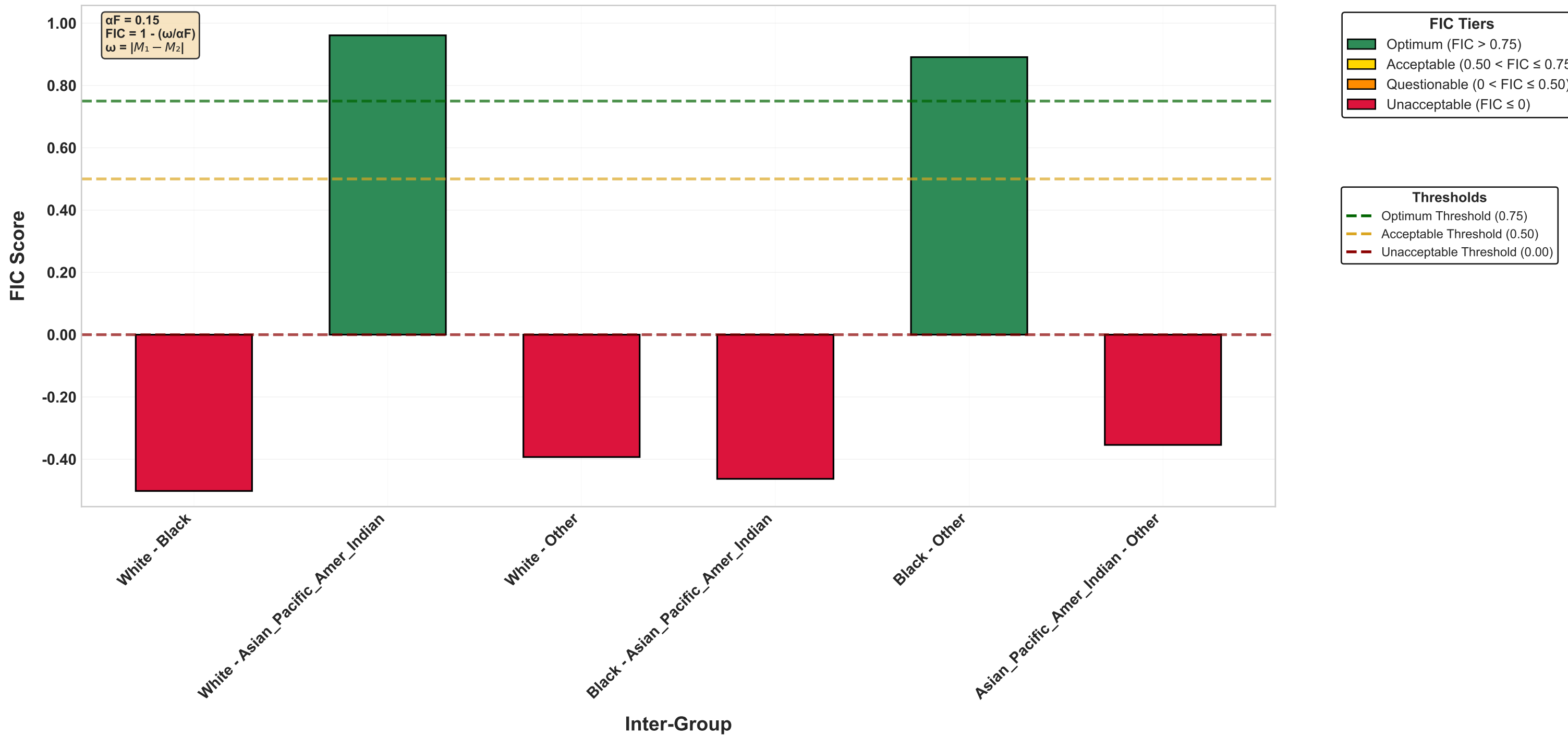
FIC Benchmarking Tiers (selection_rate, \alpha F = 0.15 )
