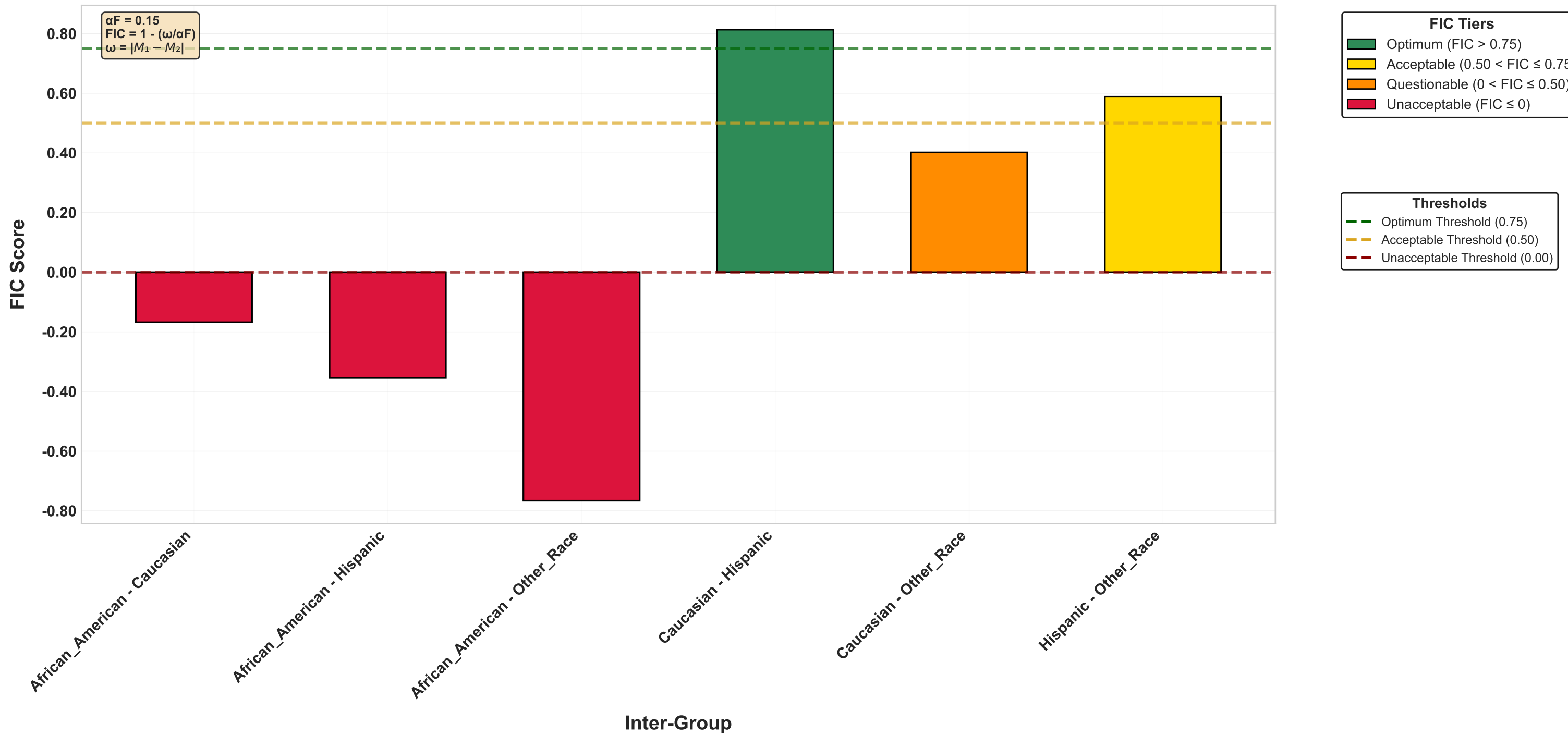
FIC Benchmarking Tiers (npv, \alpha F = 0.15 )
