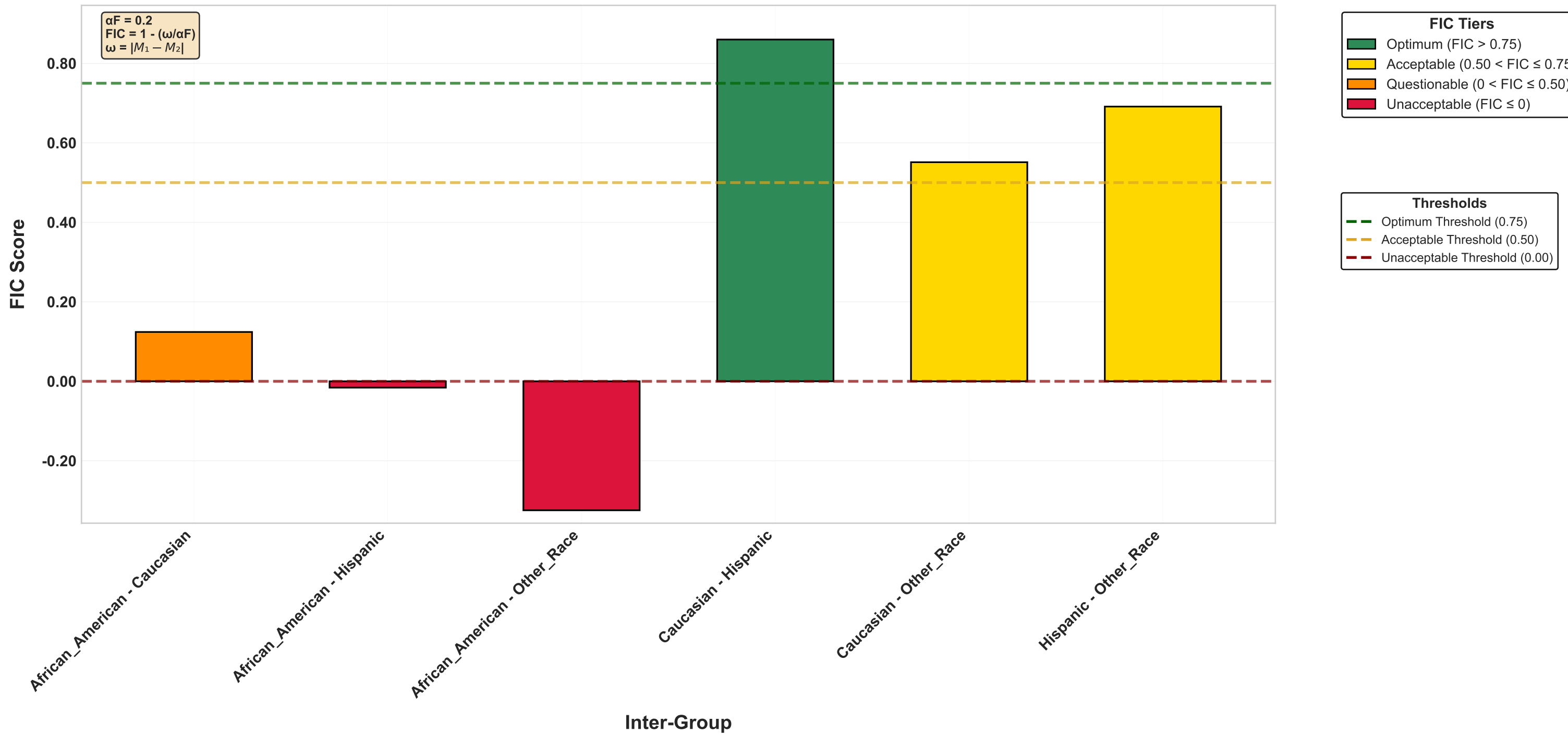
FIC Benchmarking Tiers (npv, \alpha F = 0.2 )
