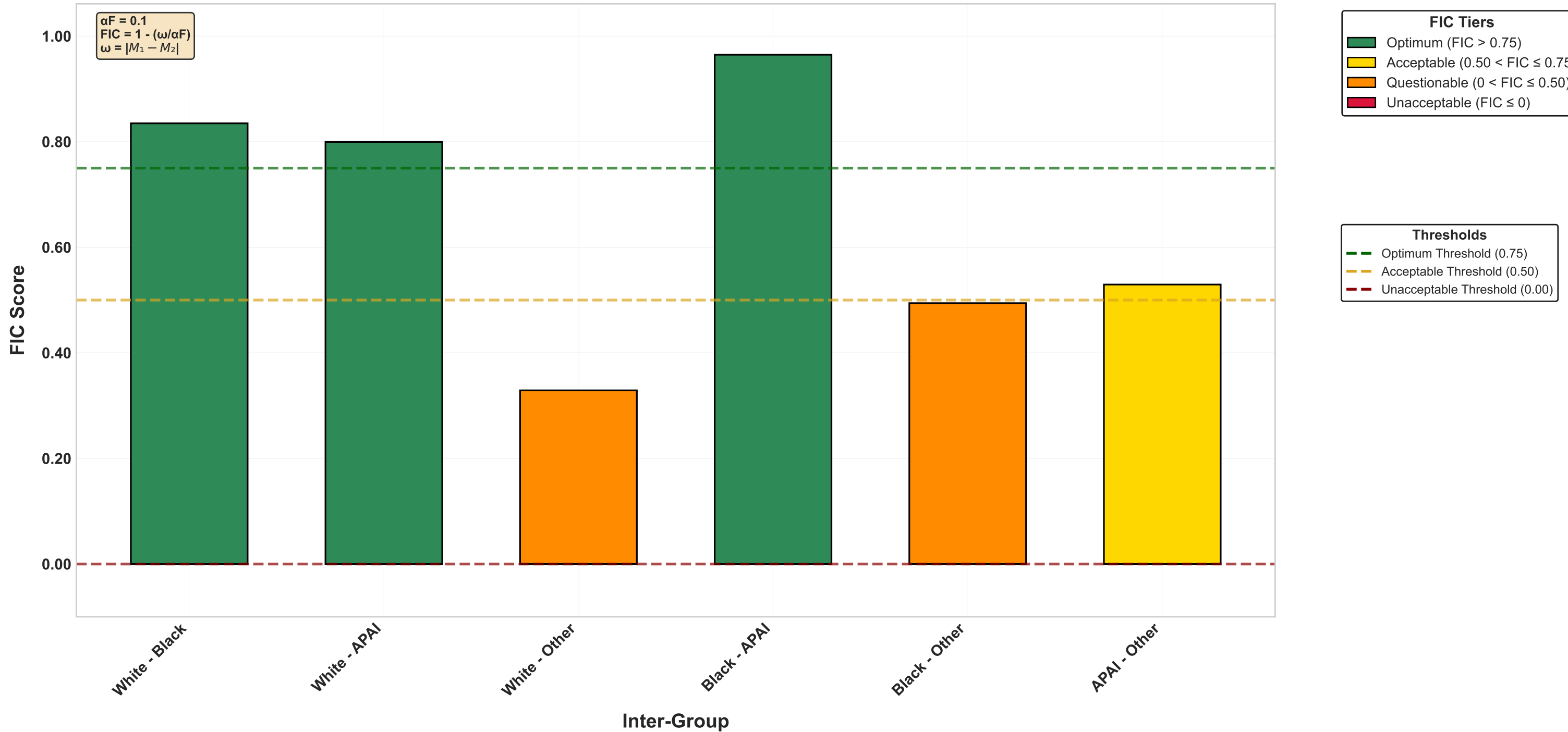
FIC Benchmarking Tiers (npv, \alpha F = 0.1 )
