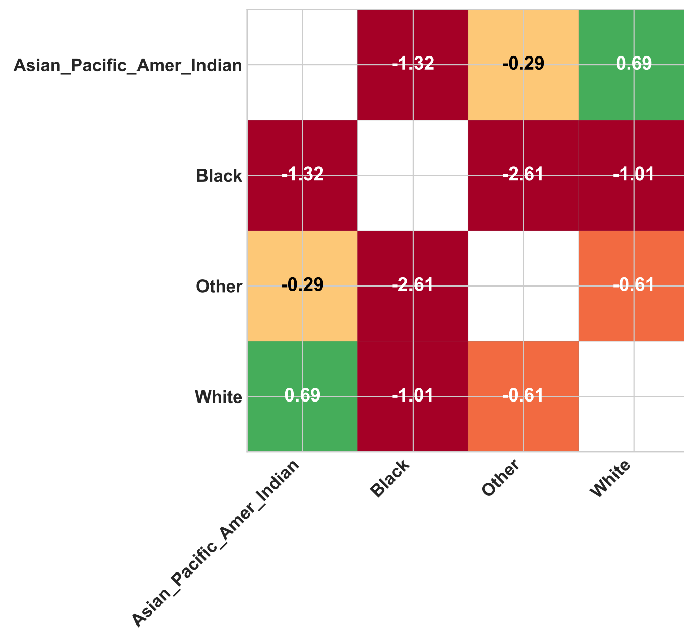
\alpha F = 0.2
