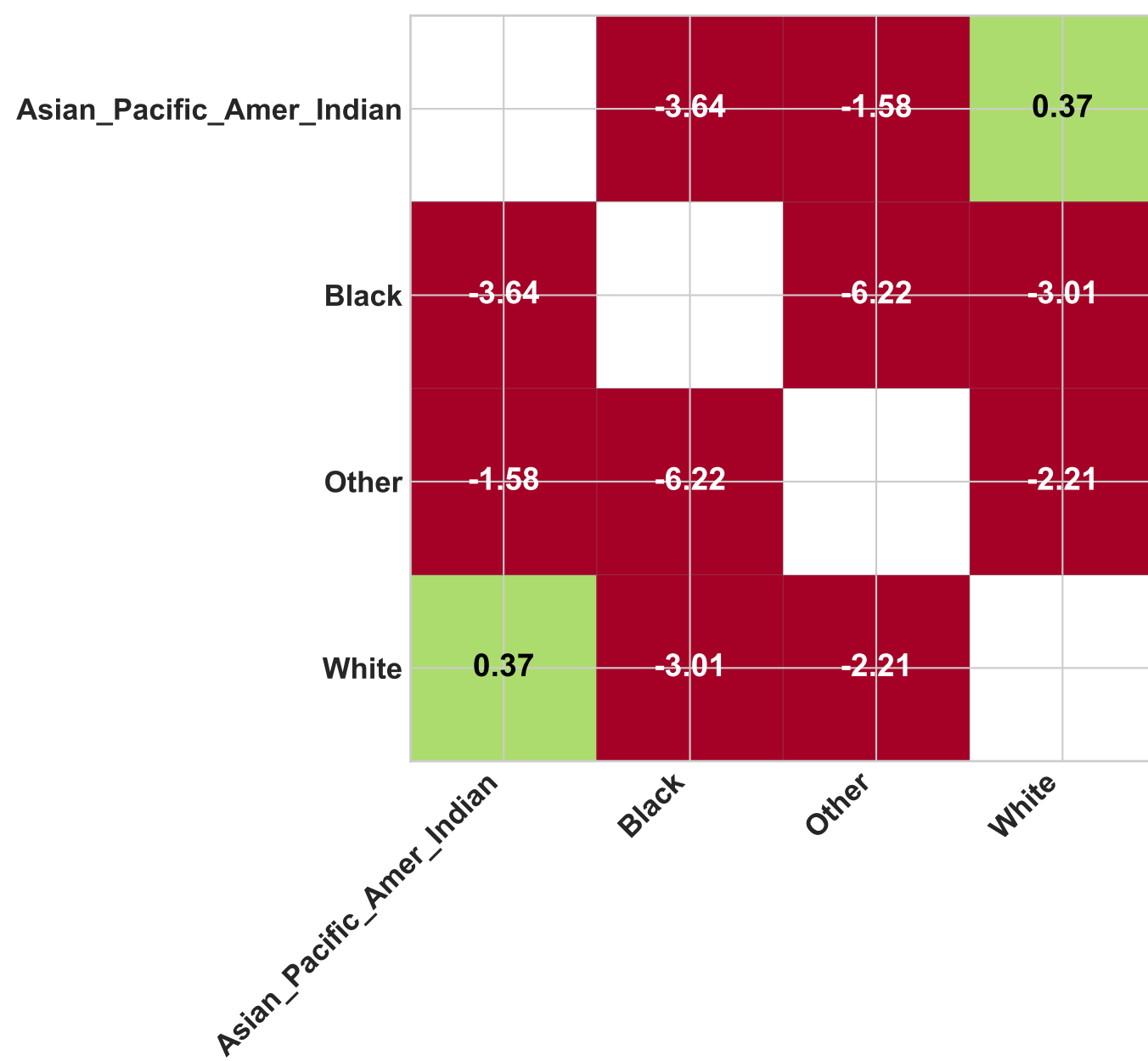
\alpha F = 0.15
