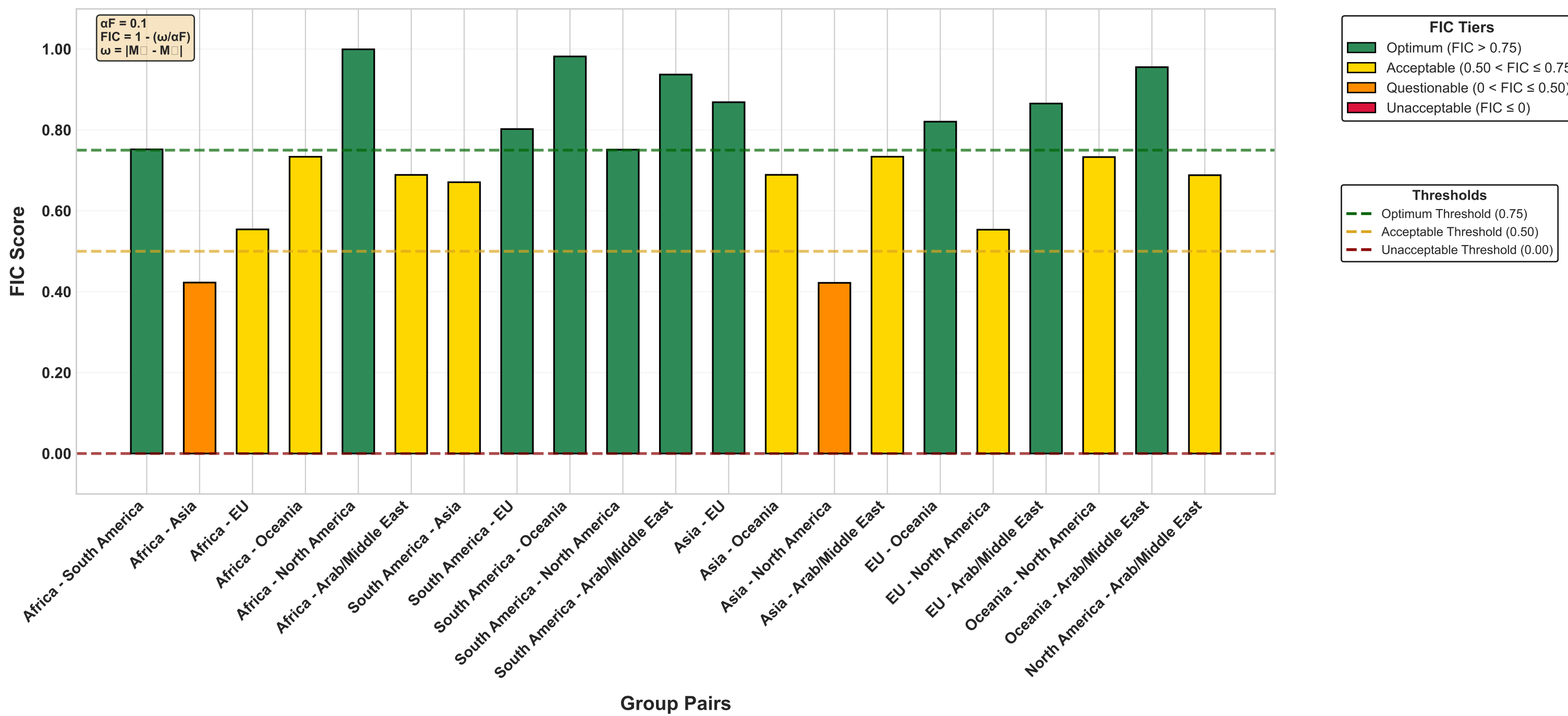
Case2_Criminal Justice - Recidivism Risk_auc FIC Benchmarking Tiers (auc, \alpha F = 0.1 )
