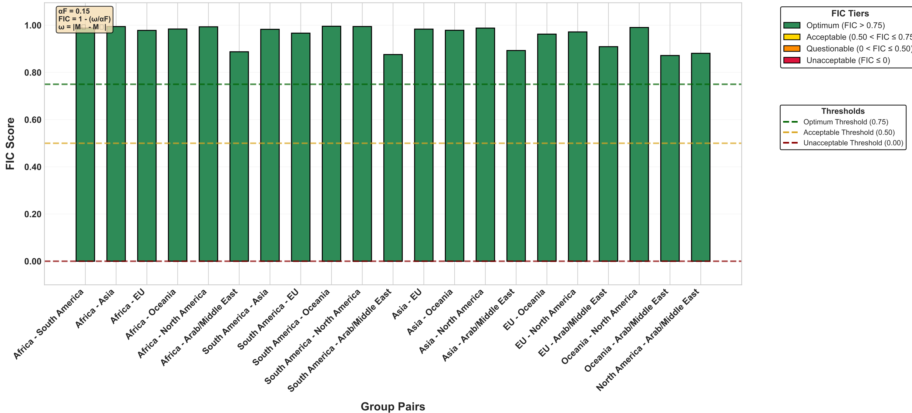
Case2_Criminal Justice - Recidivism Risk_selection_rate FIC Benchmarking Tiers (selection_rate, αF = 0.15)
