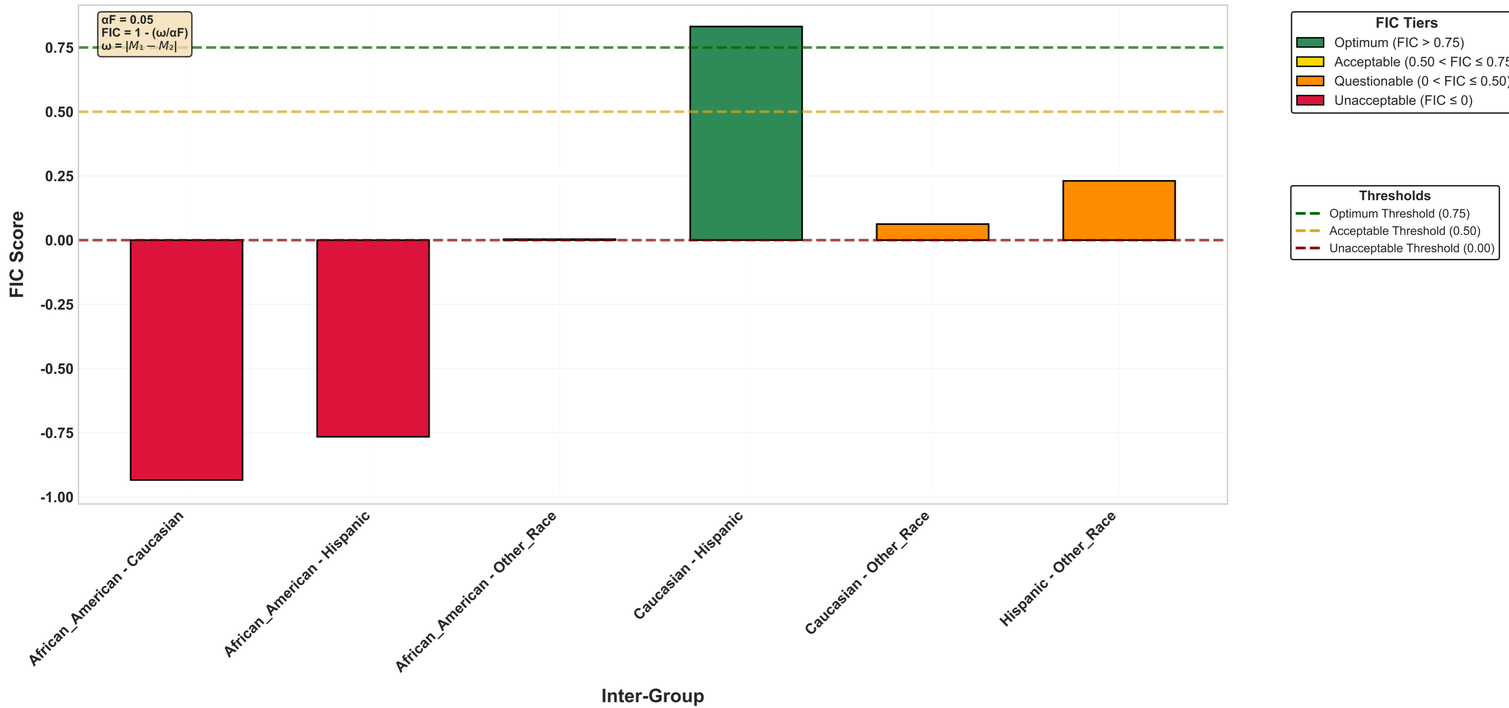
FIC Benchmarking Tiers (fnr, \alpha F = 0.05 )
