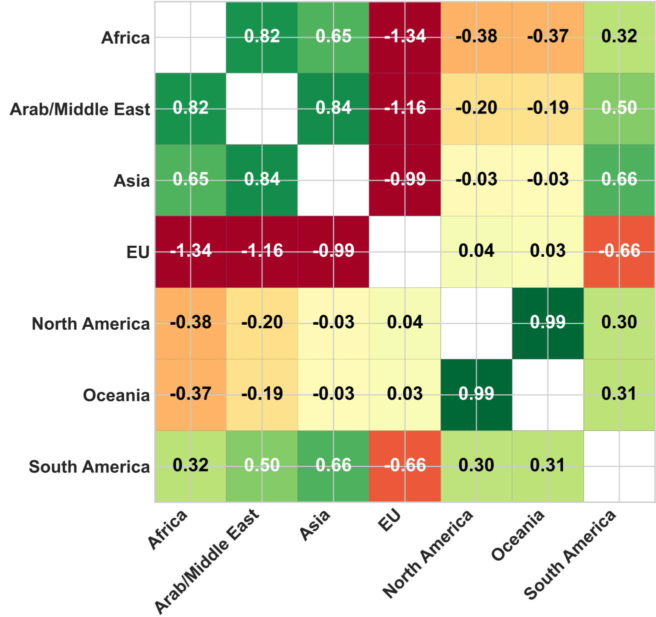
\alpha F = 0.15
