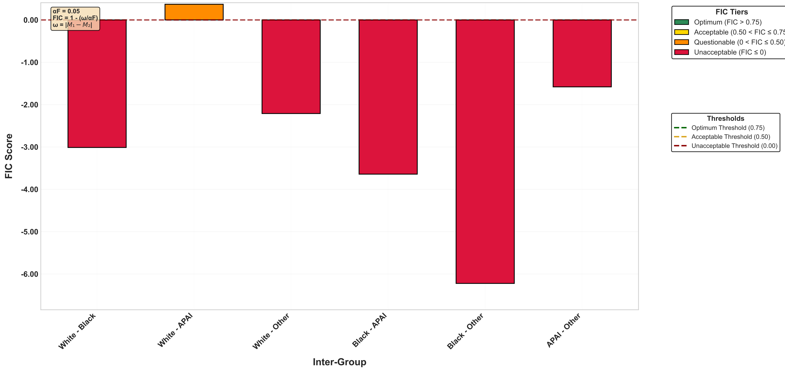
FIC Benchmarking Tiers (tpr, \alpha F = 0.05 )
