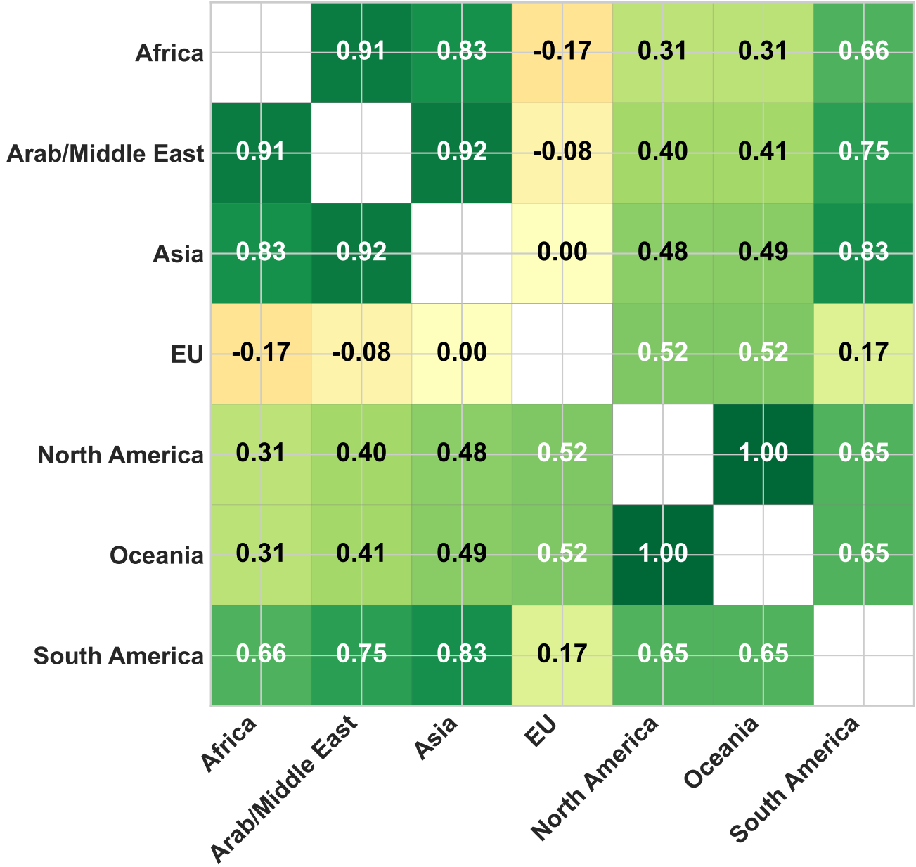
\alpha F = 0.2
