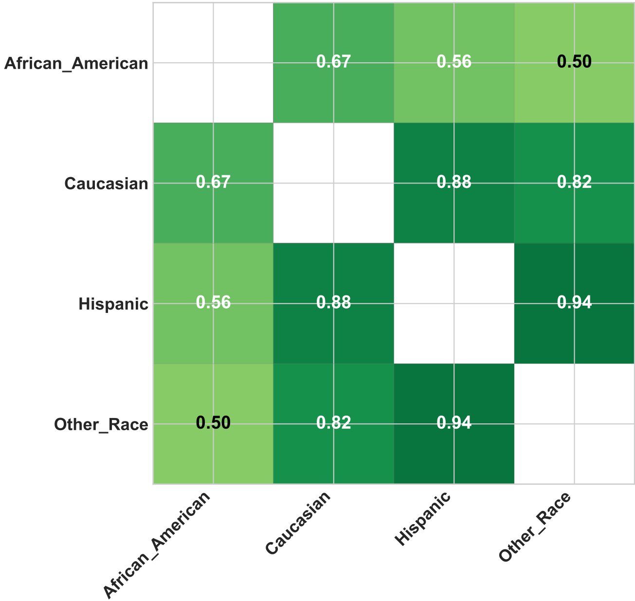
\alpha F = 0.2
