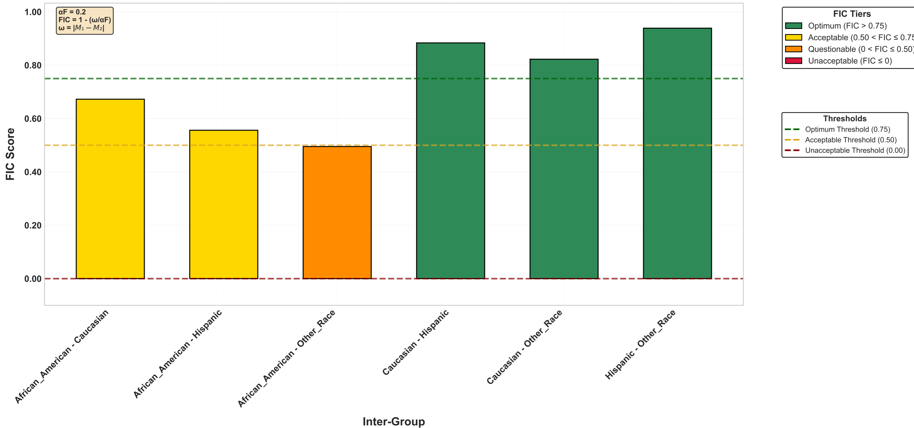
FIC Benchmarking Tiers (auc, \alpha F = 0.2 )
