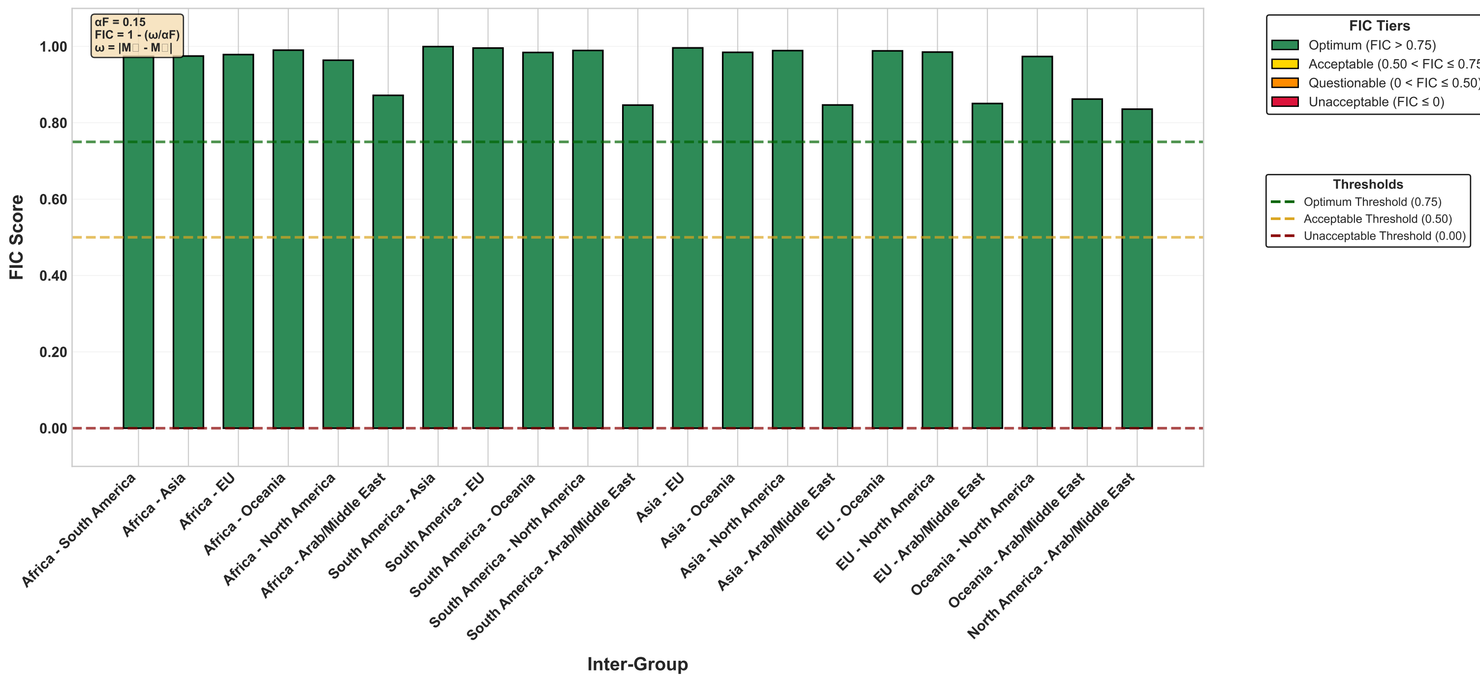
Case2_Criminal Justice - Recidivism Risk_fpr FIC Benchmarking Tiers (fpr, \alpha F = 0.15 )
