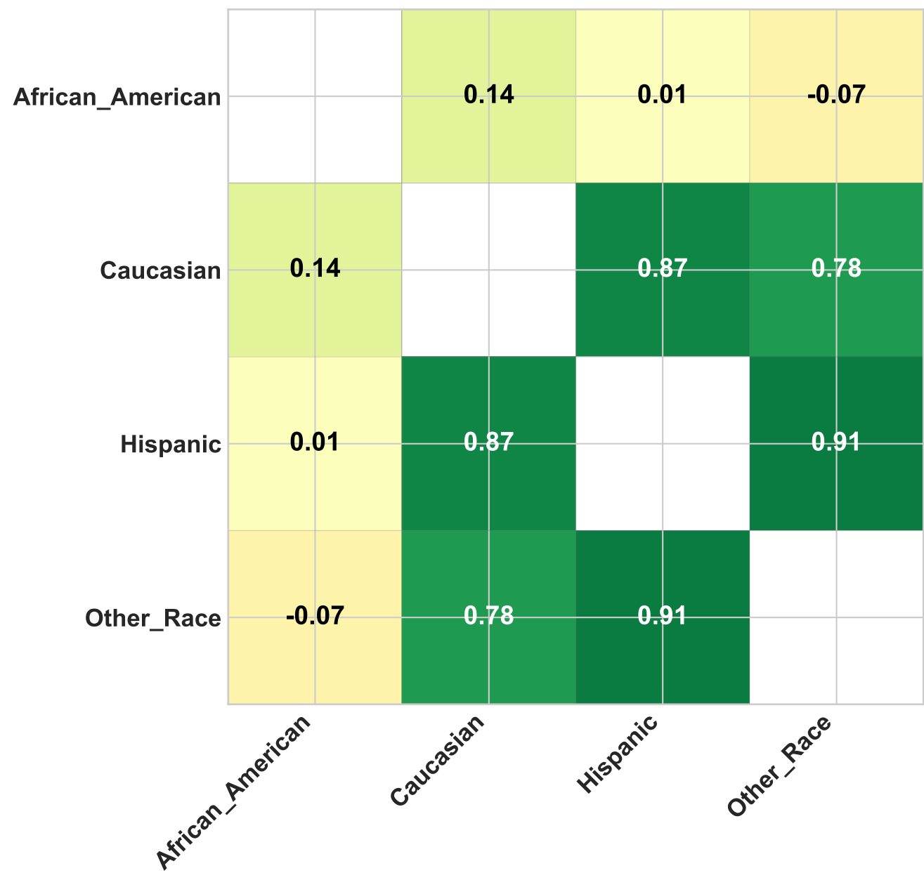
\alpha F = 0.2
