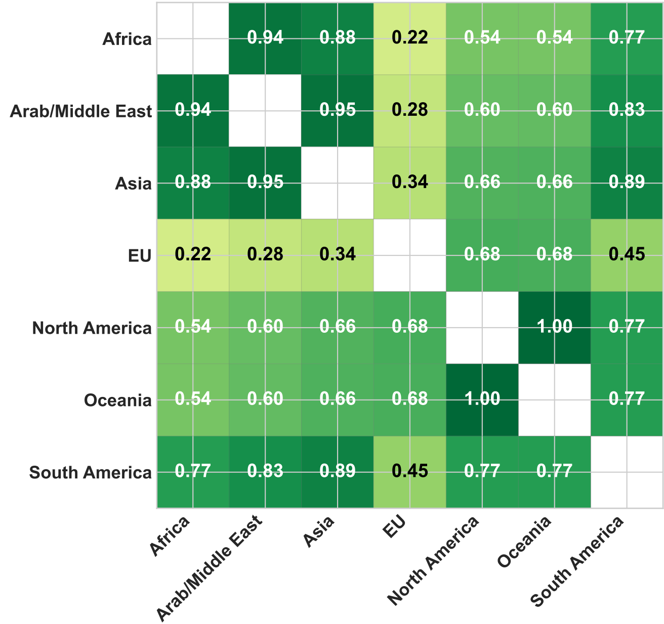
\alpha F = 0.15
