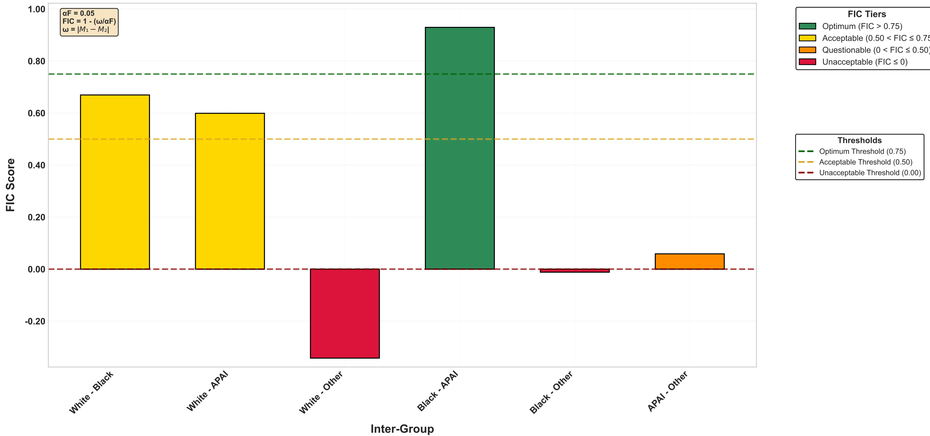
FIC Benchmarking Tiers (npv, \alpha F = 0.05 )
