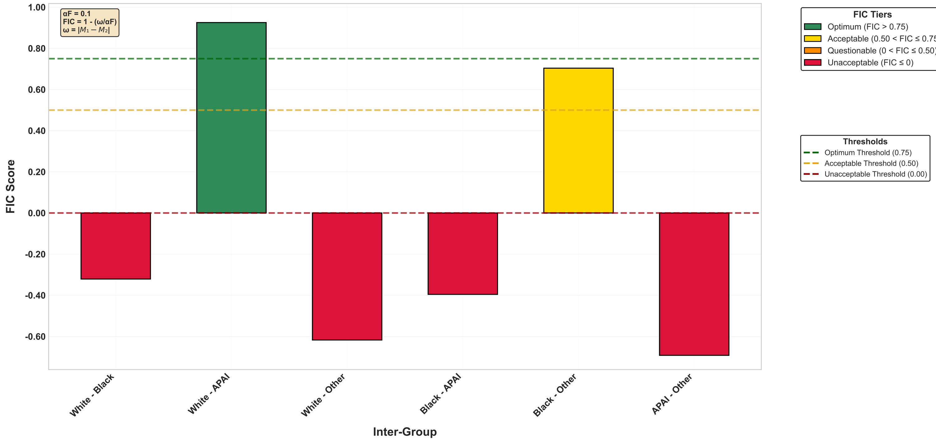
FIC Benchmarking Tiers (fpr, \alpha F = 0.1 )
