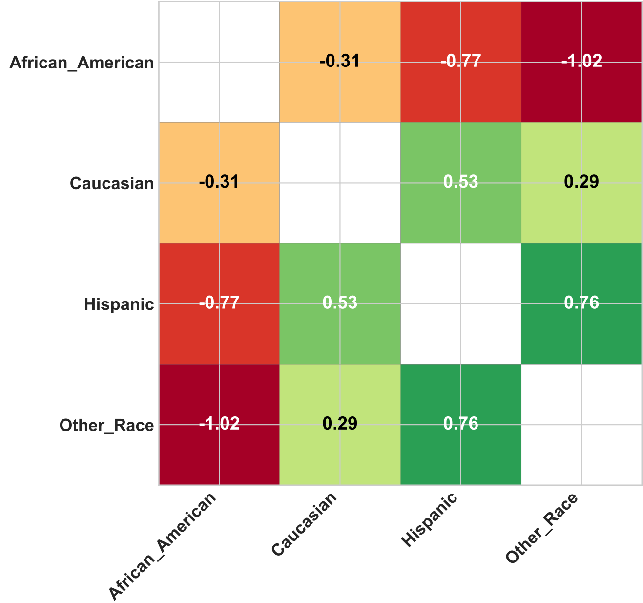
\alpha F = 0.15
