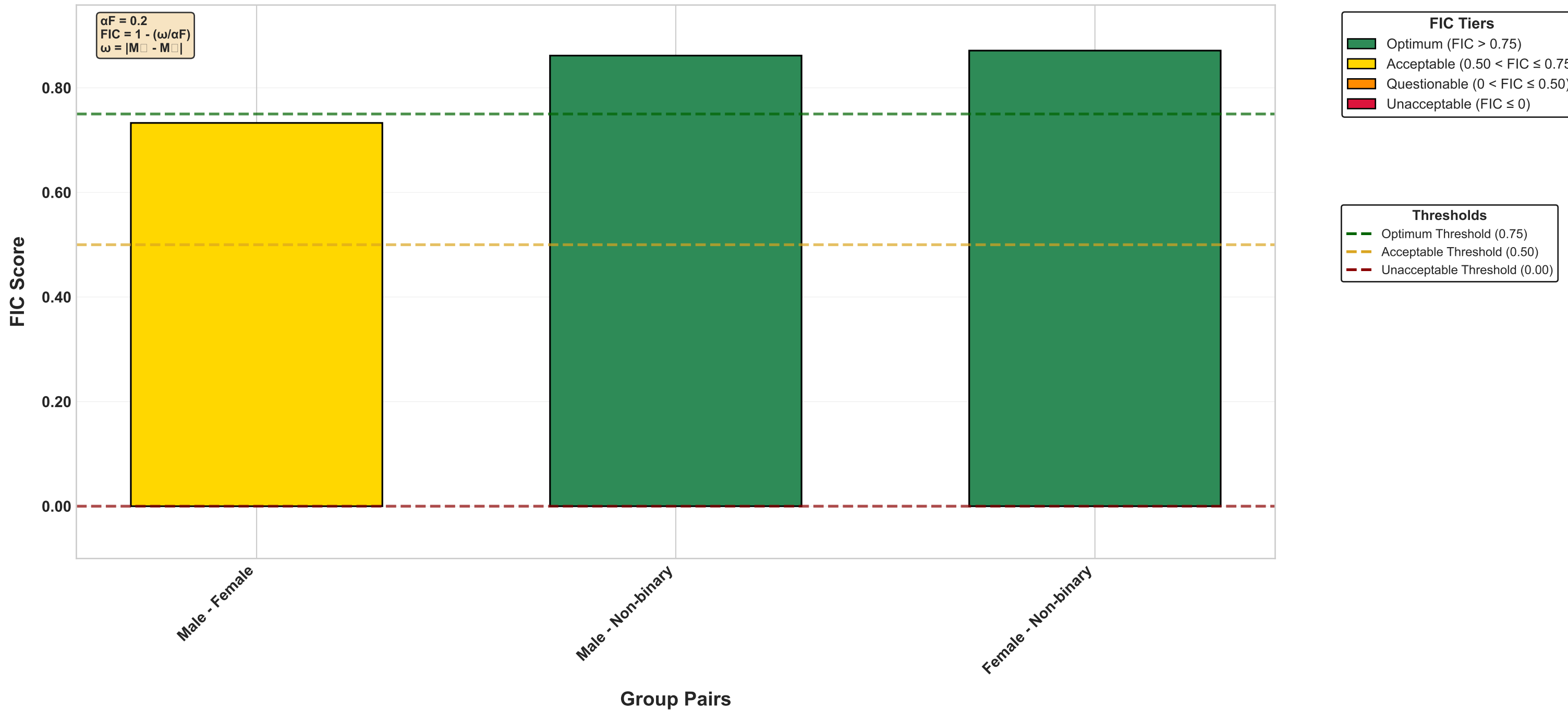
Case1_Healthcare - Depression Diagnosis_auc FIC Benchmarking Tiers (auc, \alpha F = 0.2 )
