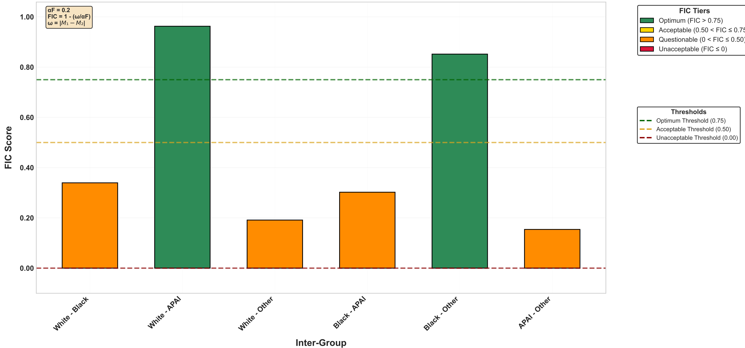
FIC Benchmarking Tiers (fpr, \alpha F = 0.2 )
