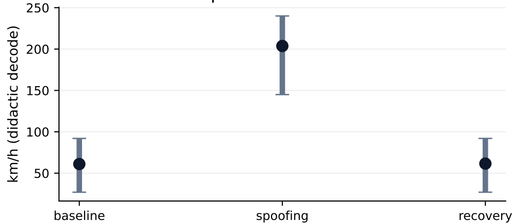
Decoded speed contrast on ID 0x100
