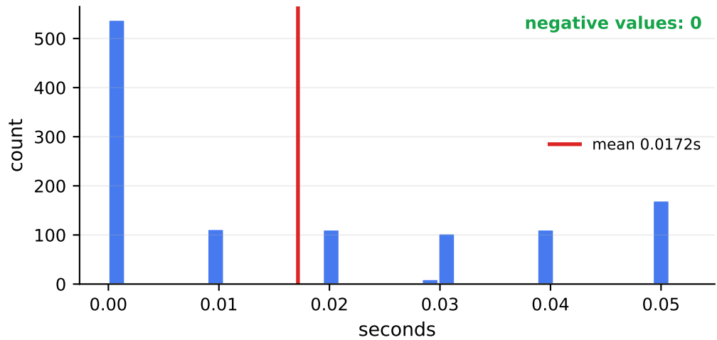
Inter-arrival distribution
