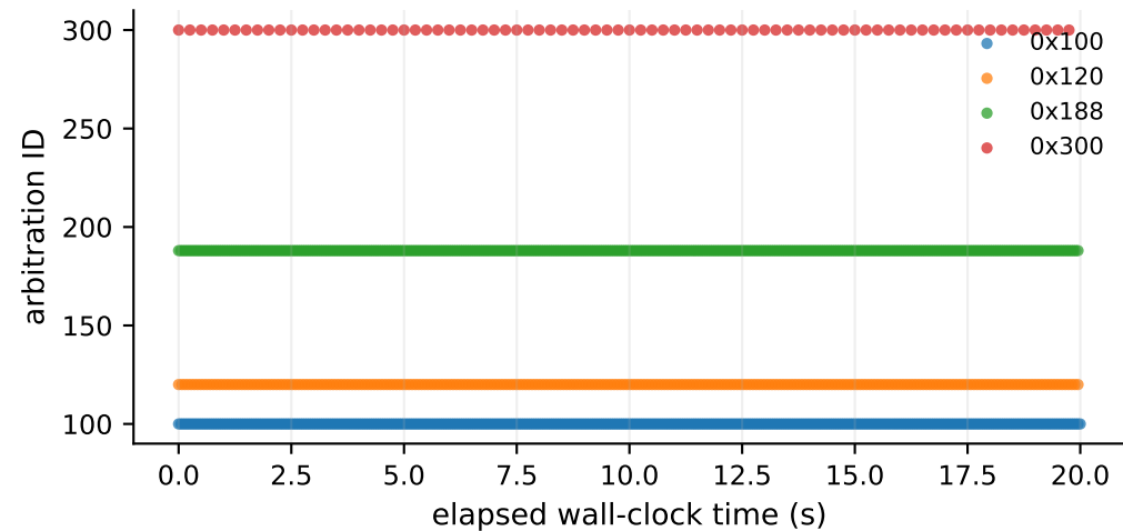
Frame timeline
