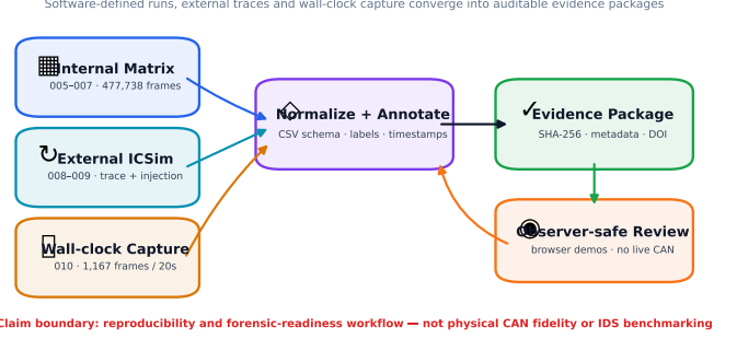
Fig. 1. Reproducible CAN evidence pipeline. Internal runs, external traces, and wall-clock capture feed a common normalization and evidence-packaging workflow with manifests, DOI-backed artifacts, and observer-safe demos.
