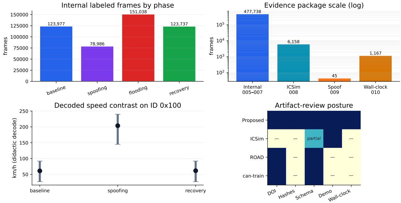
Fig. 2. Evidence coverage dashboard for the v5 artifact. The figure summarizes internal phase balance, external and injected packages, didactic speed contrast, and artifact-review posture.
