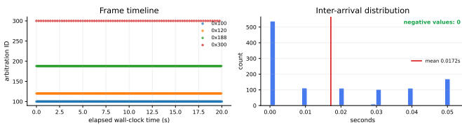
Fig. 3. Experiment 010 wall-clock timing evidence: frame timeline and inter-arrival distribution from the software-only real-time capture.
