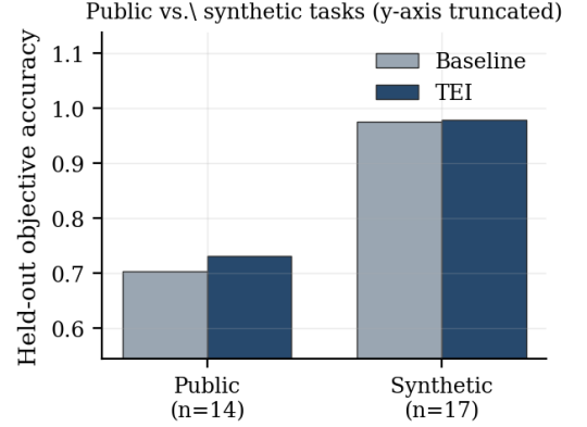
Figure 3: Left: per-task held-out objective, baseline \rightarrow TEI; ups and downs roughly balance. Right: public vs. synthetic tasks ( y -axis truncated); the baseline \rightarrow TEI movement is small in both, slightly larger on public tasks.
