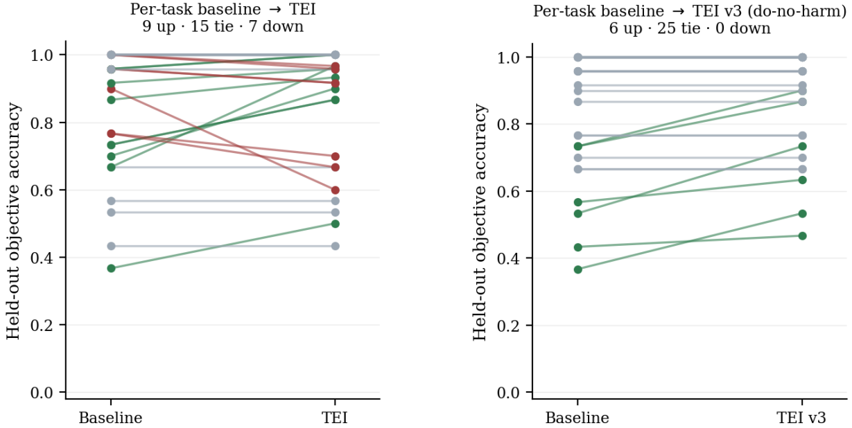
Figure 3: Why the do-no-harm gate matters (before/after). Left: naive evaluation-guided selection without a confirmation gate (the original TEI) regresses on 7 held-out tasks. These are not prompts the optimizer knowingly accepted as worse—it only keeps train-improving candidates—but a train→test generalization gap on the unseen test. Right: TEI with the do-no-harm confirmation gate ships the baseline unless a candidate is confirmed to improve an independent validation split, which eliminates all regressions (0 down) while keeping the confirmed gains.
