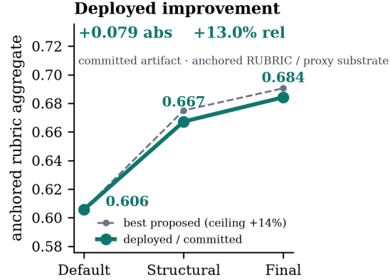
Figure 1: TEI-SWE at a glance. One structural-plus-prompt optimization loop, applied across 30 independently developed leaderboard systems, raises the deployed artifacts’ anchored rubric by 13.0% relative to baseline (RUBRIC/proxy substrate) and retains a strict blinded majority on 22 of 26 patched systems, at $1.79 LLM cost per system. Zero executed benchmark rollouts were used as the selection signal; the dashed line is the best- proposed search ceiling (14.0%), shown secondary and not necessarily committed.
