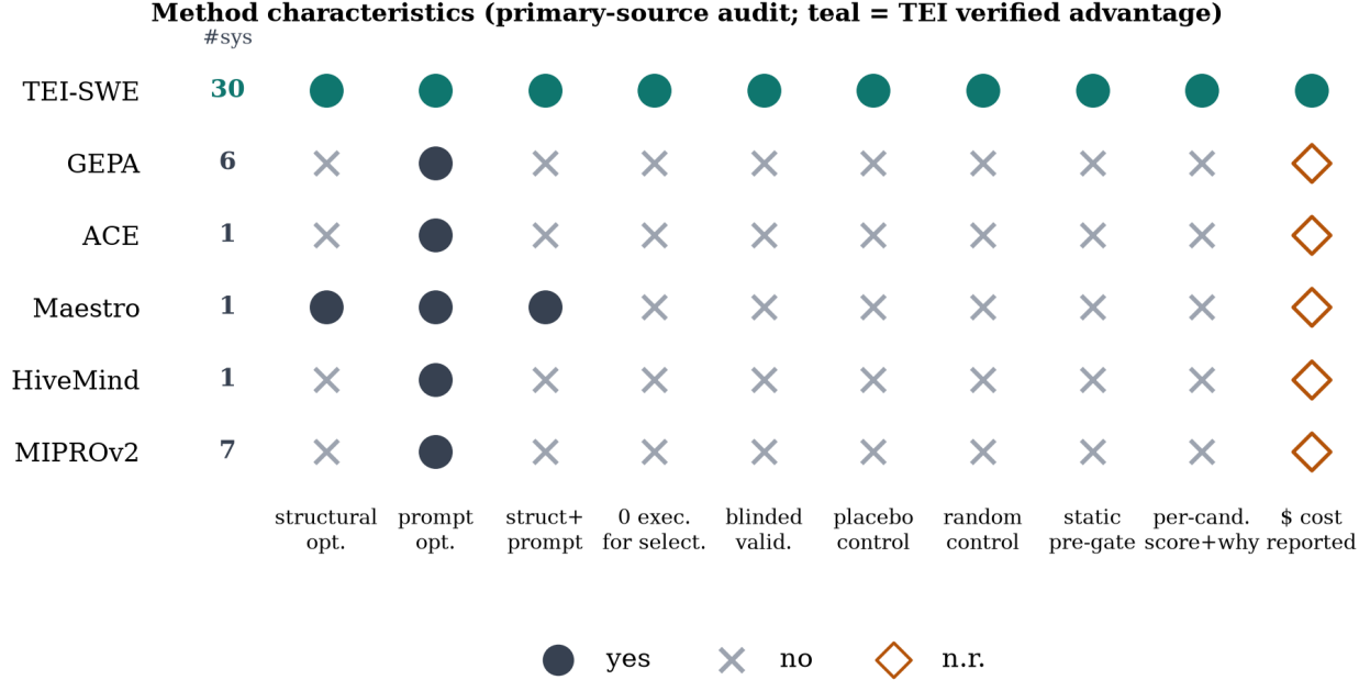
Figure 8: Where TEI differs from 2026 optimizers. TEI differs primarily in third-party-system coverage, structural-plus-prompt scope, zero-executed-rollout proxy selection, and bias-controlled validation; performance numbers are not compared across incompatible substrates. Filled teal marks a primary-source-verified TEI advantage on the audited axis; “n.r.” (open diamond) means not reported and is never encoded as “no.”
