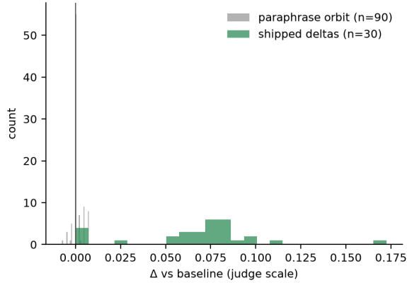
Figure 6: Shipped deltas (green) vs. the paraphrase orbit (gray) over 90 paraphrases (RUBRIC rung): directed proposals separate cleanly from rewording noise.
