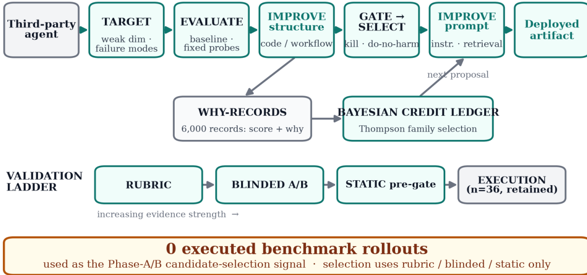
Figure 3: How TEI works. A per-agent loop targets the weakest rubric dimension, then improves both the structural (code/workflow) and prompt surfaces under sequential gating (futility, posterior kill, do-no-harm), while a Bayesian credit ledger steers the next proposal from the 6,000 score+why records. No executed benchmark rollout is used as the Phase-A/B candidate-selection signal—selection runs on the anchored rubric, blinded A/B, and static checks; execution ( n=36 , retained) is a separate downstream rung.
