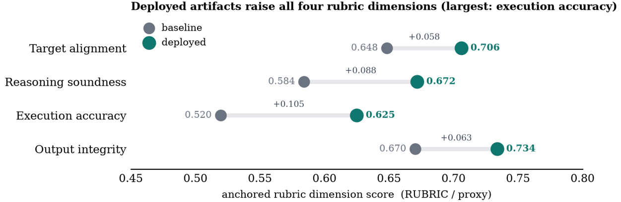
Figure 5: TEI’s deployed artifacts increase all four anchored rubric dimensions on the 26 patched systems; execution accuracy—the weakest dimension at baseline for all 30 systems—shows the largest absolute gain (+0.105, RUBRIC/proxy substrate).
