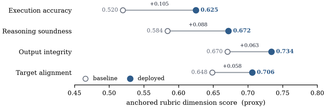
Figure 5: TEI’s deployed artifacts increase all four anchored rubric dimensions on the 26 patched systems (rows ordered by absolute deployed gain, largest first); execution accuracy—the weakest dimension at baseline for all 30 systems—shows the largest gain (+0.105, RUBRIC/proxy substrate).
