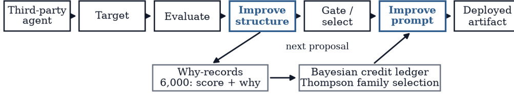
Phase-A/B candidate selection uses the rubric, blinded A/B and static checks only — no executed benchmark rollouts.
