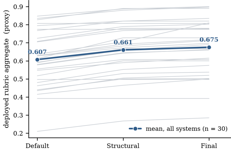
Figure 4: Deployed trajectories for all 30 systems (thin gray) and their mean (RUBRIC rung). Population = all 30, so the mean ends at the all-30 deployed final (0.675), lower than the n=26 patched headline (0.684) because the four flat trajectories are the zero-patch null-control systems. Structural dominates; prompt adds a residual.
