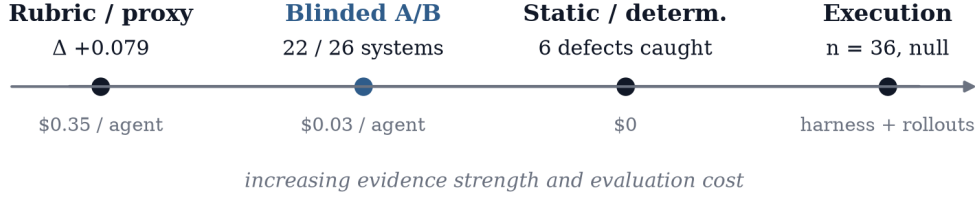
Figure 2: The validation ladder. Four rungs of increasing evidence strength and marginal cost; a claim is only as strong as the highest rung it reaches. This study climbs all four: anchored rubric ( \Delta +0.079 on the patched n=26 ), blinded A/B (22/26 systems), zero-cost static checks (six defects caught), and a retained n=36 execution arm (null). Every outcome-facing claim is carried by the blinded rung, not by rubric magnitudes.
