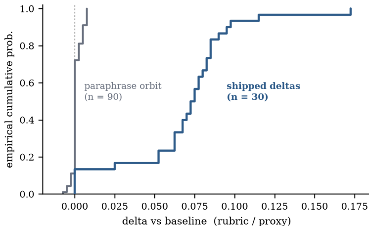
Figure 6: Paired empirical CDFs (RUBRIC rung): the 90 paraphrase rewordings pile up at zero while the 30 shipped deployed deltas are shifted right, separating cleanly from rewording noise. ECDFs normalise the unequal sample sizes ( n=90 vs. n=30 ) and span 0–1, so there is no raw-count-axis distortion.
