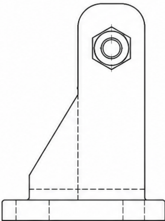
RIGHT VIEW
