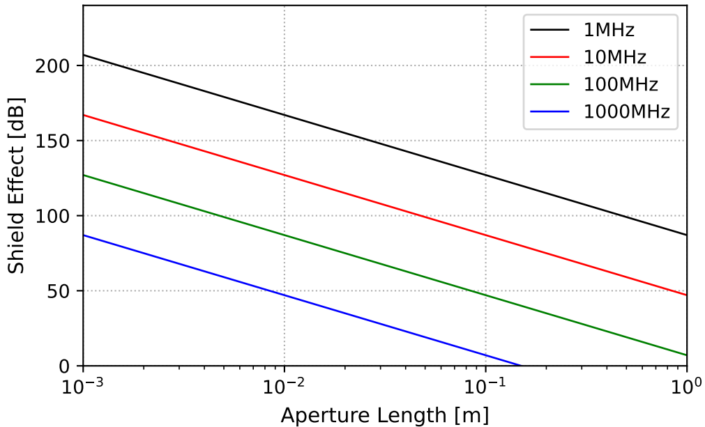
Shield Effect of a Round Aperture
