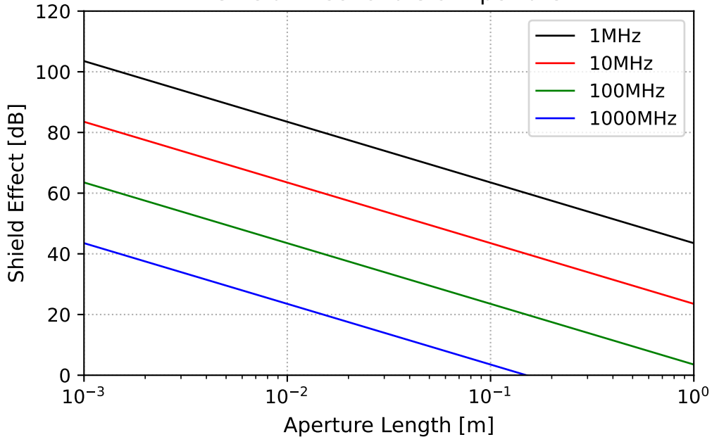
Shield Effect of a Slot Aperture
