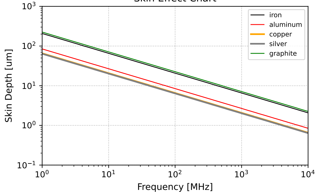
Skin Effect Chart
