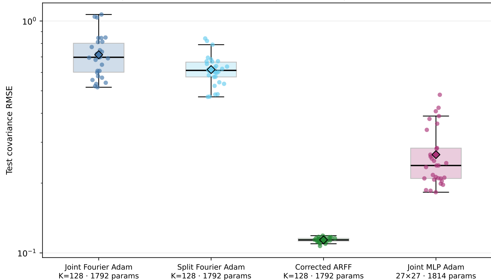
Experiment 8: covariance recovery at matched parameter count
